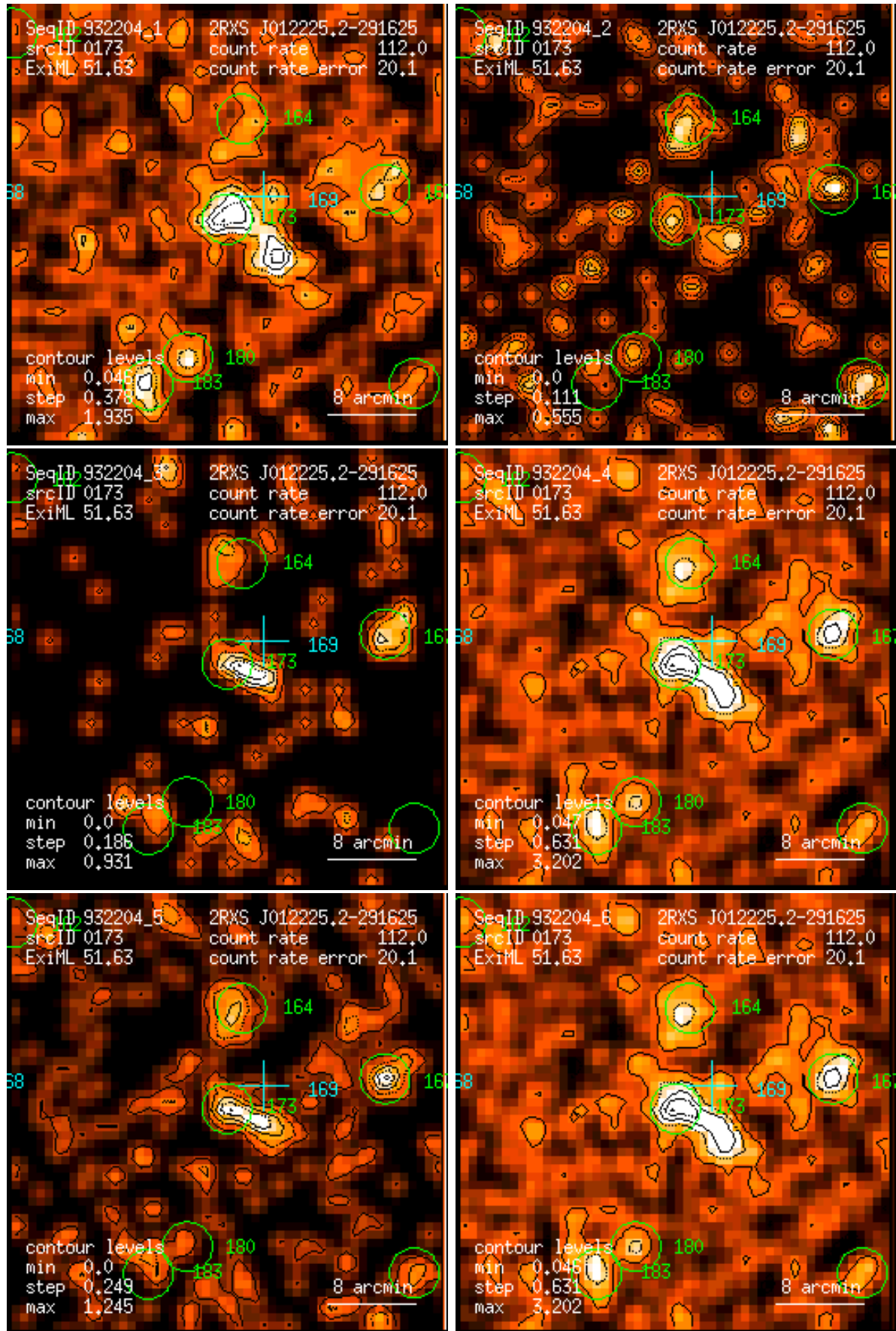
Figure 173: RASS 932204: detection 0173: band rate images, Gaussian filter: (1) PSPC channels 11 – 41, (2) 52 – 90, (3) 91 – 201, (4) 11 – 235, (5) 52 – 201, (6) 11 – 201. Broad band rates in counts/ks. Band rate contour levels in counts/ks/arcmin 2 .
