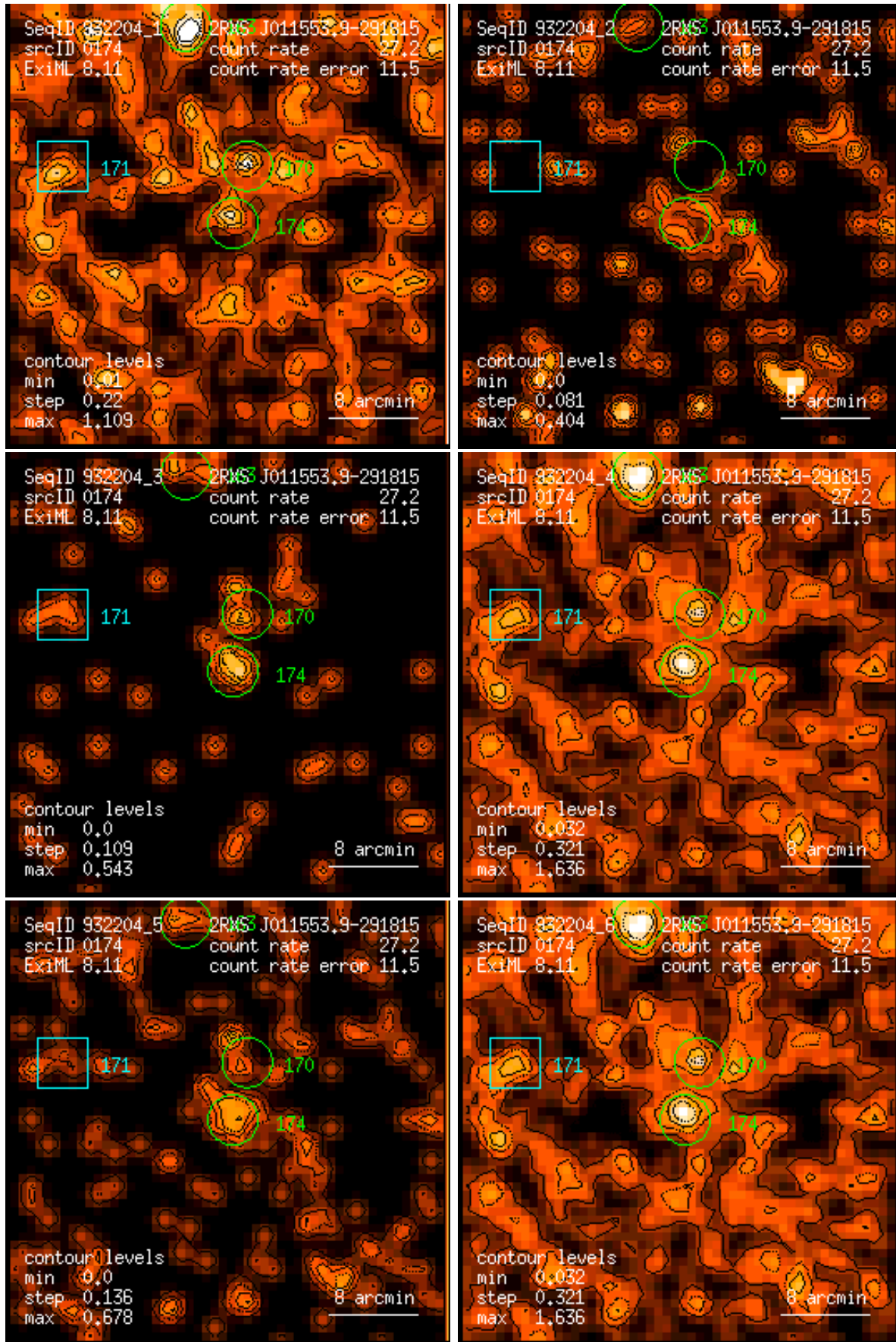
Figure 174: RASS 932204: detection 0174: band rate images, Gaussian filter: (1) PSPC channels 11 – 41, (2) 52 – 90, (3) 91 – 201, (4) 11 – 235, (5) 52 – 201, (6) 11 – 201. Broad band rates in counts/ks. Band rate contour levels in counts/ks/arcmin 2 .
