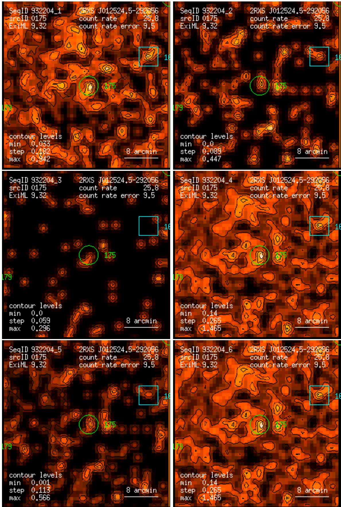
Figure 175: RASS 932204: detection 0175: band rate images, Gaussian filter: (1) PSPC channels 11 – 41, (2) 52 – 90, (3) 91 – 201, (4) 11 – 235, (5) 52 – 201, (6) 11 – 201. Broad band rates in counts/ks. Band rate contour levels in counts/ks/arcmin 2 .
