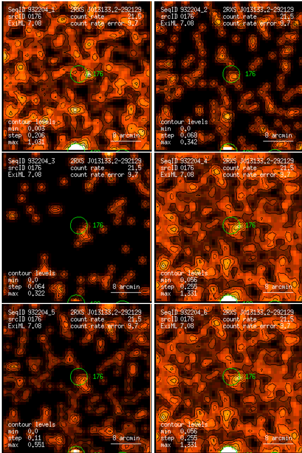
Figure 176: RASS 932204: detection 0176: band rate images, Gaussian filter: (1) PSPC channels 11 – 41, (2) 52 – 90, (3) 91 – 201, (4) 11 – 235, (5) 52 – 201, (6) 11 – 201. Broad band rates in counts/ks. Band rate contour levels in counts/ks/arcmin 2 .
