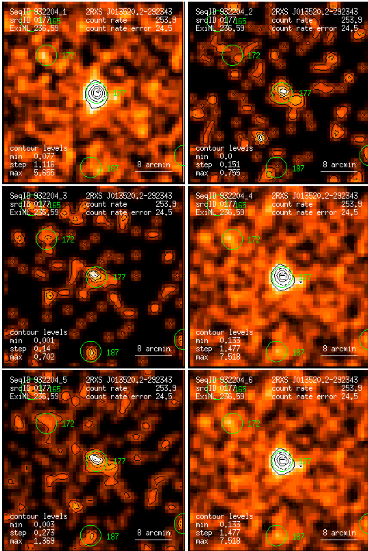
Figure 177: RASS 932204: detection 0177: band rate images, Gaussian filter: (1) PSPC channels 11 – 41, (2) 52 – 90, (3) 91 – 201, (4) 11 – 235, (5) 52 – 201, (6) 11 – 201. Broad band rates in counts/ks. Band rate contour levels in counts/ks/arcmin 2 .
