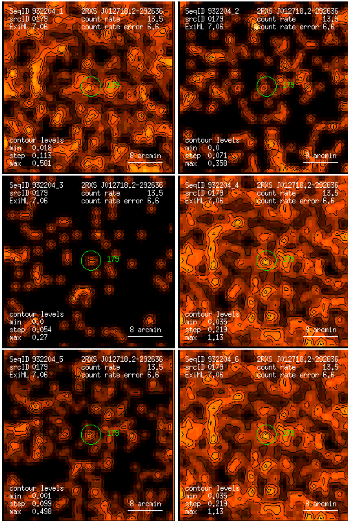
Figure 179: RASS 932204: detection 0179: band rate images, Gaussian filter: (1) PSPC channels 11 – 41, (2) 52 – 90, (3) 91 – 201, (4) 11 – 235, (5) 52 – 201, (6) 11 – 201. Broad band rates in counts/ks. Band rate contour levels in counts/ks/arcmin 2 .
