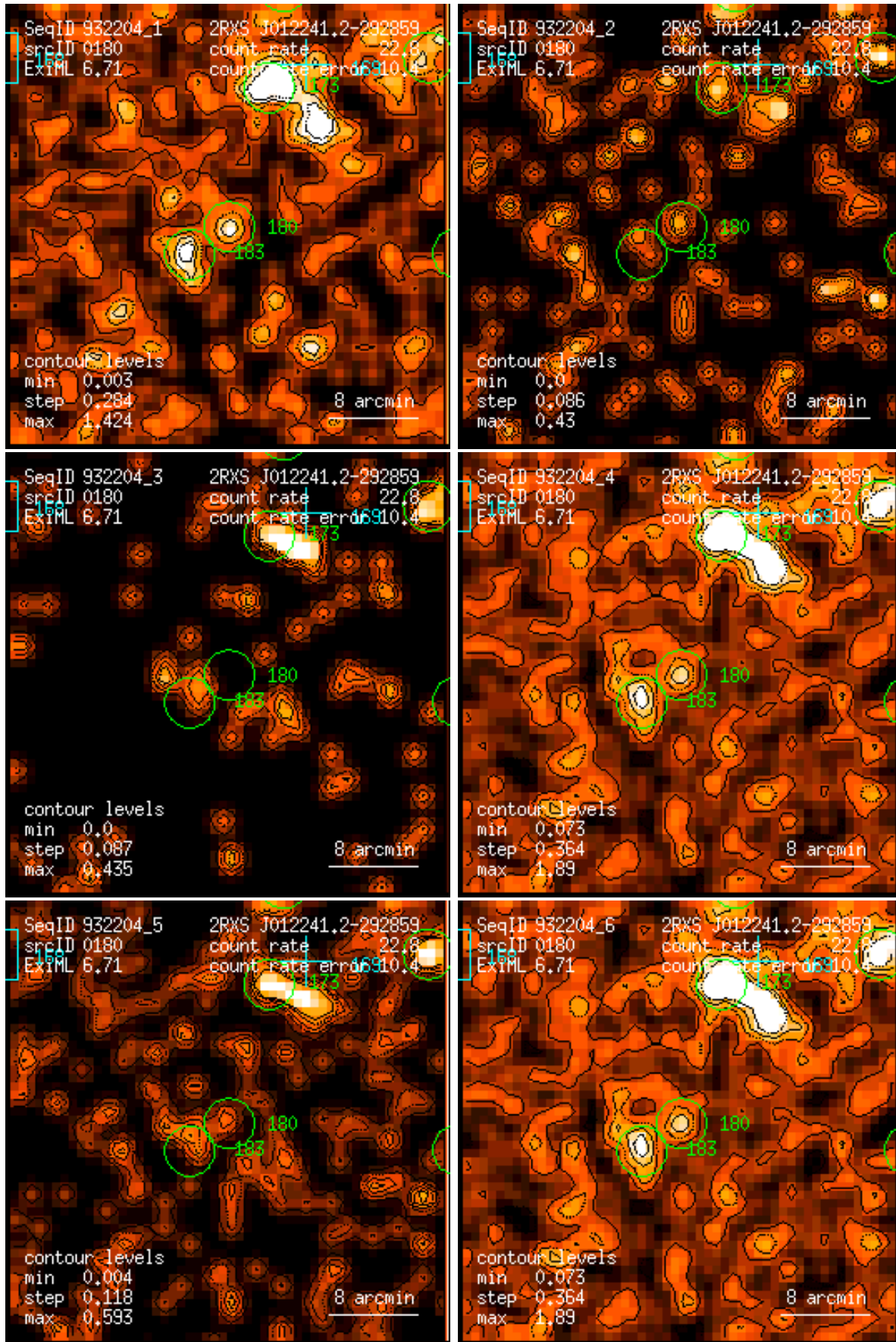
Figure 180: RASS 932204: detection 0180: band rate images, Gaussian filter: (1) PSPC channels 11 – 41, (2) 52 – 90, (3) 91 – 201, (4) 11 – 235, (5) 52 – 201, (6) 11 – 201. Broad band rates in counts/ks. Band rate contour levels in counts/ks/arcmin 2 .
