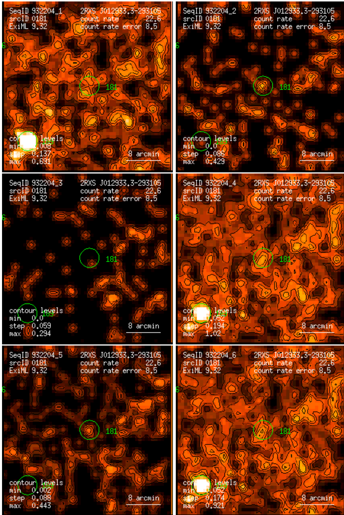
Figure 181: RASS 932204: detection 0181: band rate images, Gaussian filter: (1) PSPC channels 11 – 41, (2) 52 – 90, (3) 91 – 201, (4) 11 – 235, (5) 52 – 201, (6) 11 – 201. Broad band rates in counts/ks. Band rate contour levels in counts/ks/arcmin 2 .
