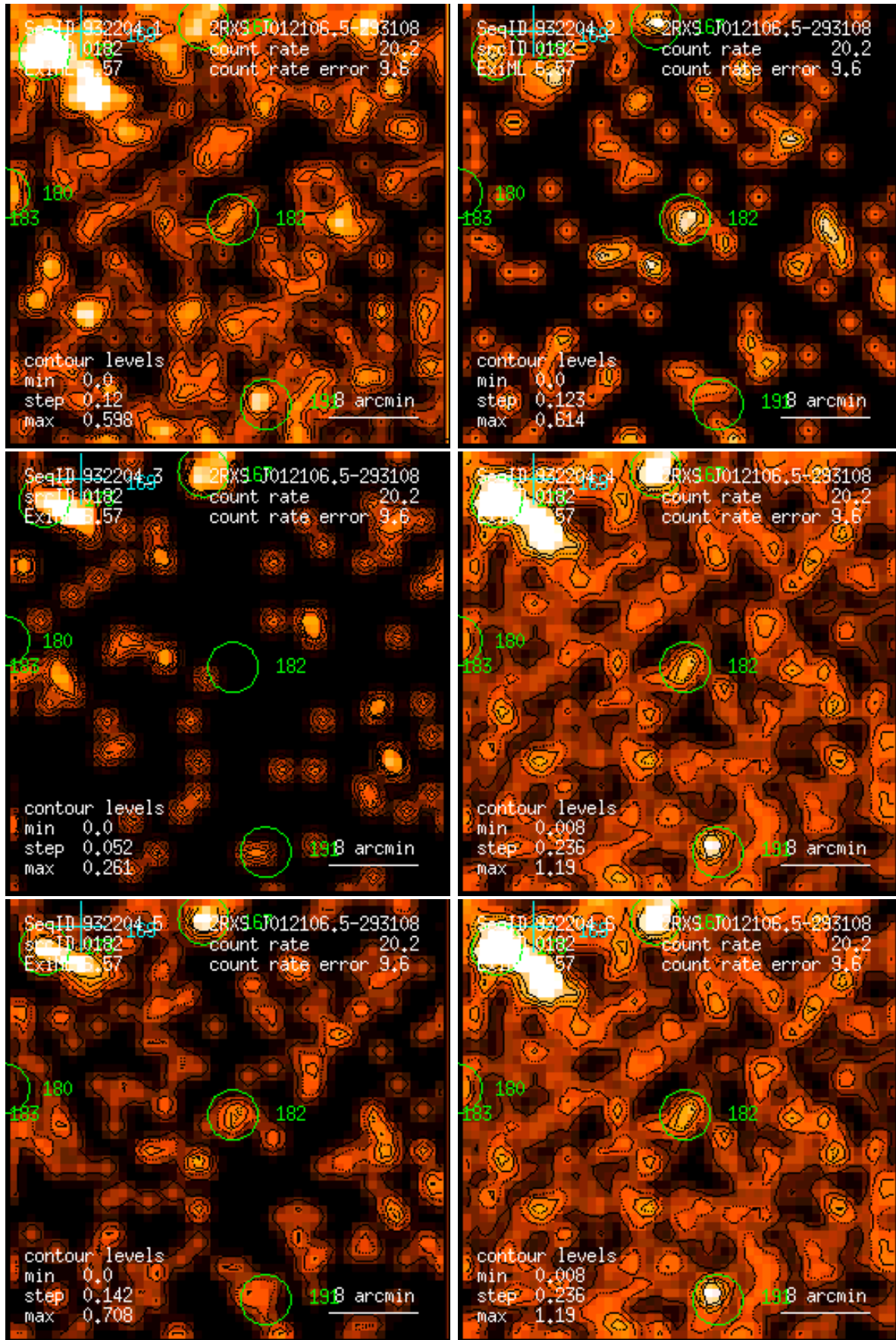
Figure 182: RASS 932204: detection 0182: band rate images, Gaussian filter: (1) PSPC channels 11 – 41, (2) 52 – 90, (3) 91 – 201, (4) 11 – 235, (5) 52 – 201, (6) 11 – 201. Broad band rates in counts/ks. Band rate contour levels in counts/ks/arcmin 2 .
