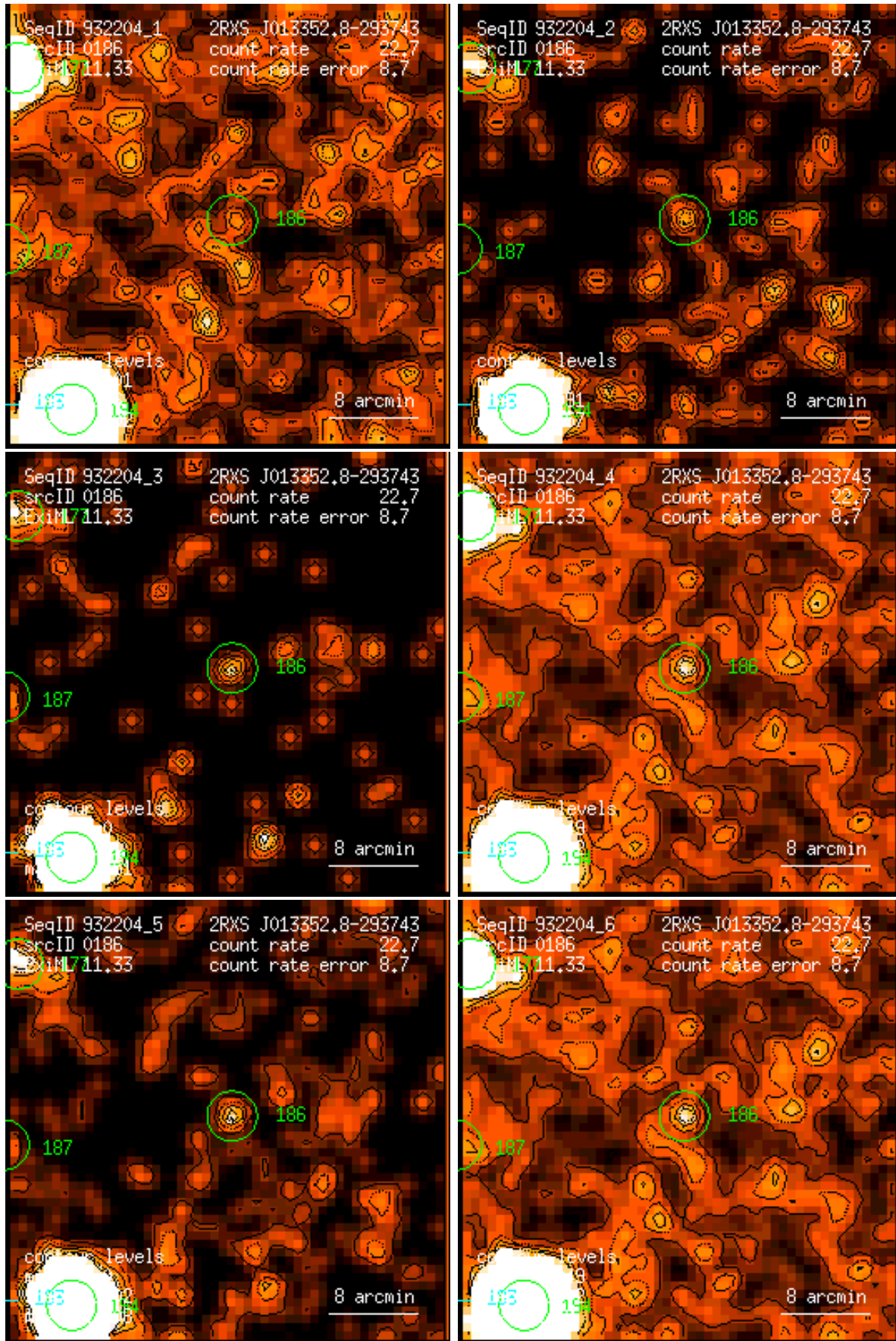
Figure 186: RASS 932204: detection 0186: band rate images, Gaussian filter: (1) PSPC channels 11 – 41, (2) 52 – 90, (3) 91 – 201, (4) 11 – 235, (5) 52 – 201, (6) 11 – 201. Broad band rates in counts/ks. Band rate contour levels in counts/ks/arcmin 2 .
