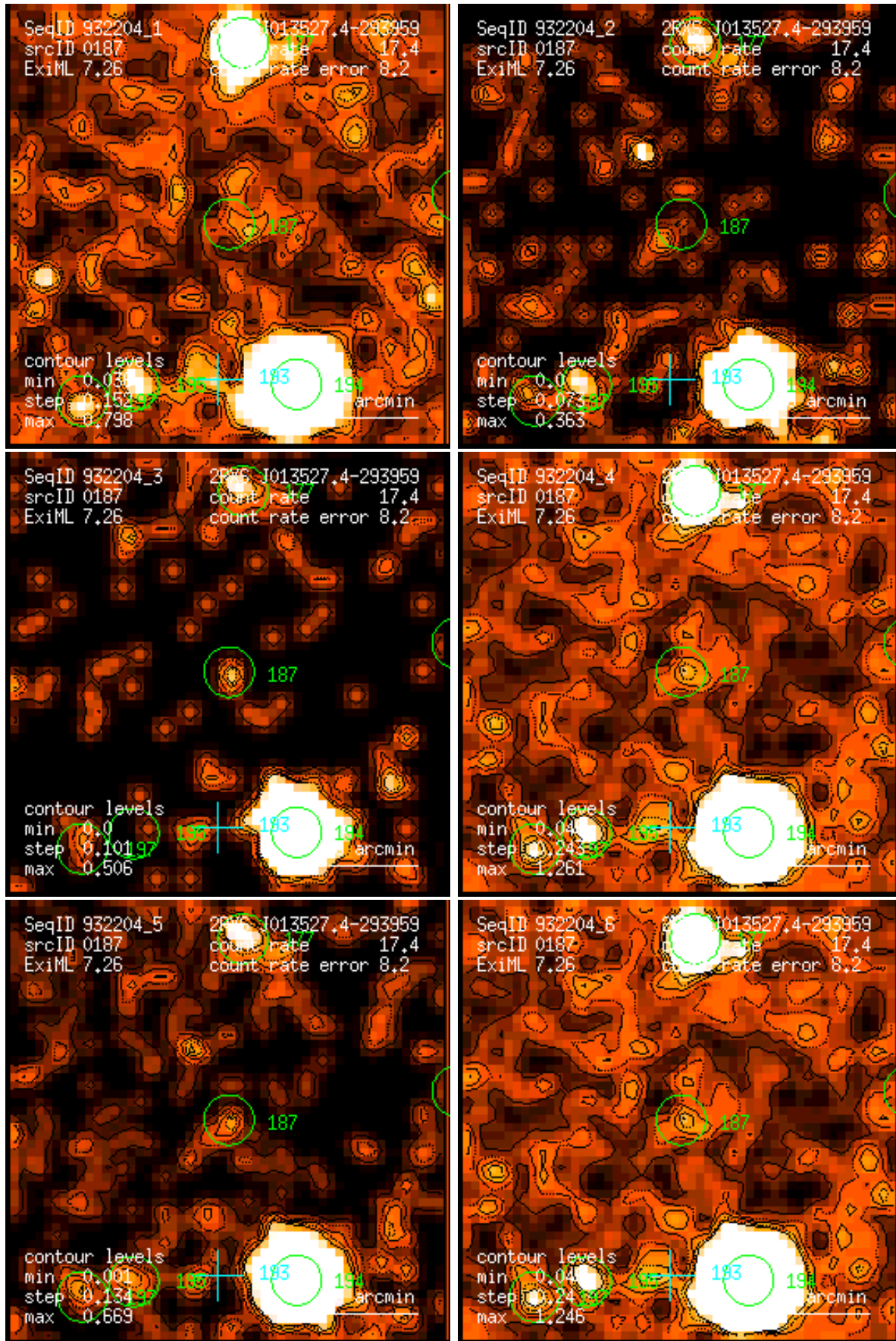
Figure 187: RASS 932204: detection 0187: band rate images, Gaussian filter: (1) PSPC channels 11 – 41, (2) 52 – 90, (3) 91 – 201, (4) 11 – 235, (5) 52 – 201, (6) 11 – 201. Broad band rates in counts/ks. Band rate contour levels in counts/ks/arcmin 2 .
