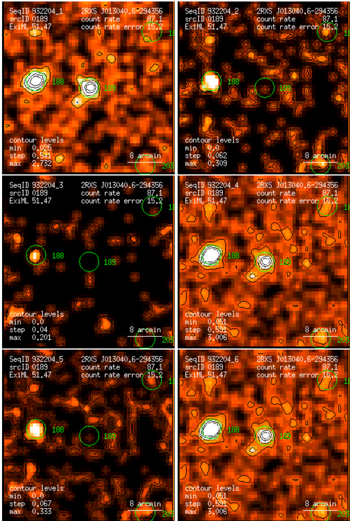
Figure 189: RASS 932204: detection 0189: band rate images, Gaussian filter: (1) PSPC channels 11 – 41, (2) 52 – 90, (3) 91 – 201, (4) 11 – 235, (5) 52 – 201, (6) 11 – 201. Broad band rates in counts/ks. Band rate contour levels in counts/ks/arcmin 2 .
