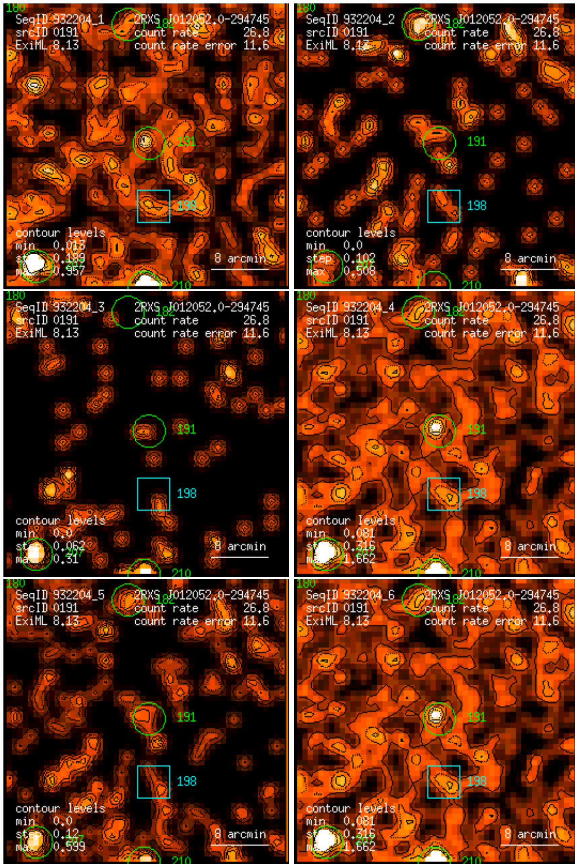
Figure 191: RASS 932204: detection 0191: band rate images, Gaussian filter: (1) PSPC channels 11 – 41, (2) 52 – 90, (3) 91 – 201, (4) 11 – 235, (5) 52 – 201, (6) 11 – 201. Broad band rates in counts/ks. Band rate contour levels in counts/ks/arcmin 2 .
