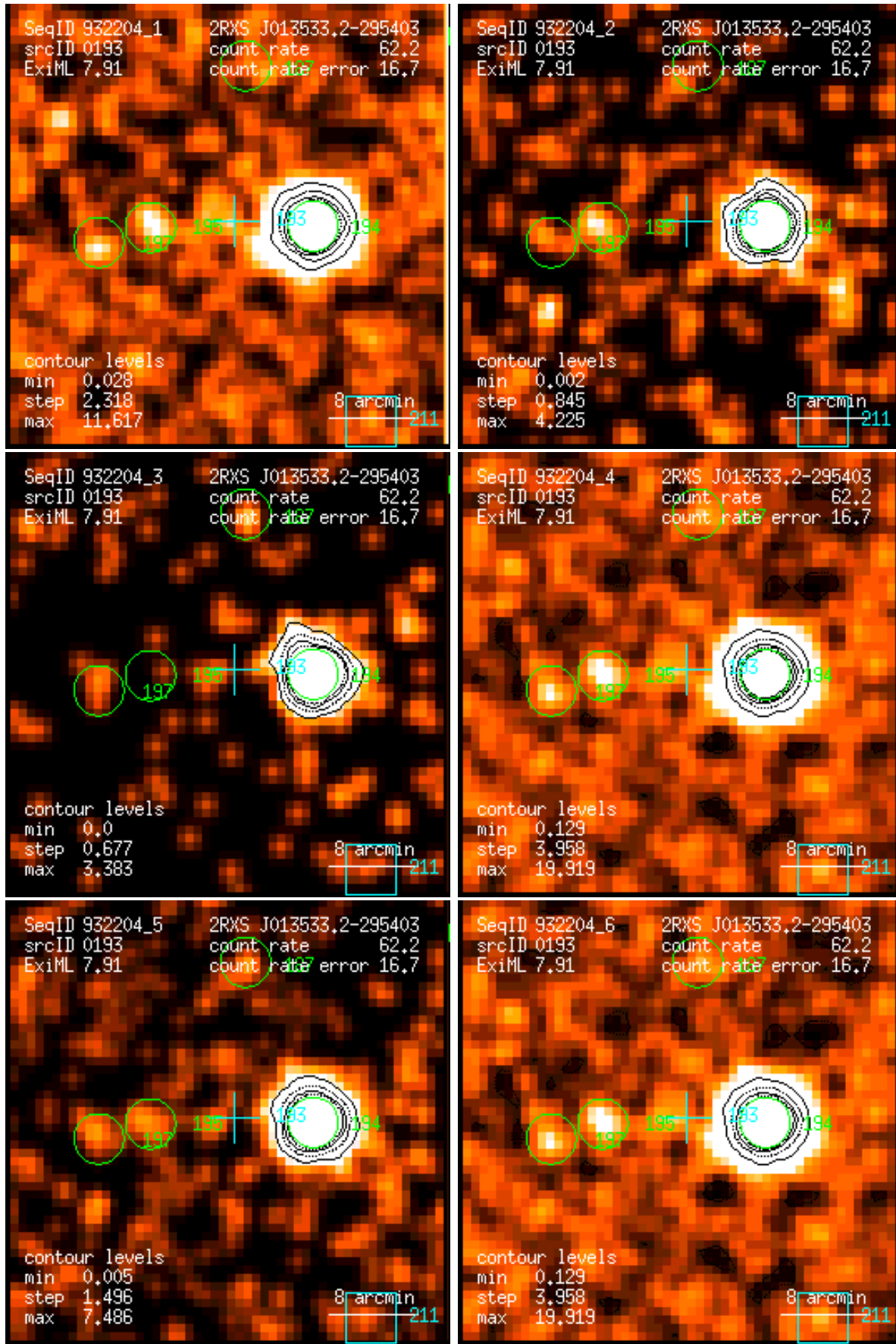
Figure 193: RASS 932204: detection 0193: band rate images, Gaussian filter: (1) PSPC channels 11 – 41, (2) 52 – 90, (3) 91 – 201, (4) 11 – 235, (5) 52 – 201, (6) 11 – 201. Broad band rates in counts/ks. Band rate contour levels in counts/ks/arcmin 2 .
