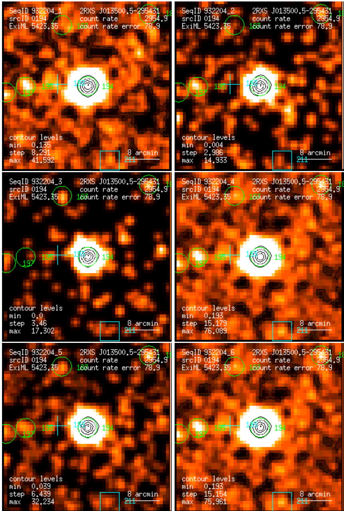
Figure 194: RASS 932204: detection 0194: band rate images, Gaussian filter: (1) PSPC channels 11 – 41, (2) 52 – 90, (3) 91 – 201, (4) 11 – 235, (5) 52 – 201, (6) 11 – 201. Broad band rates in counts/ks. Band rate contour levels in counts/ks/arcmin 2 .
