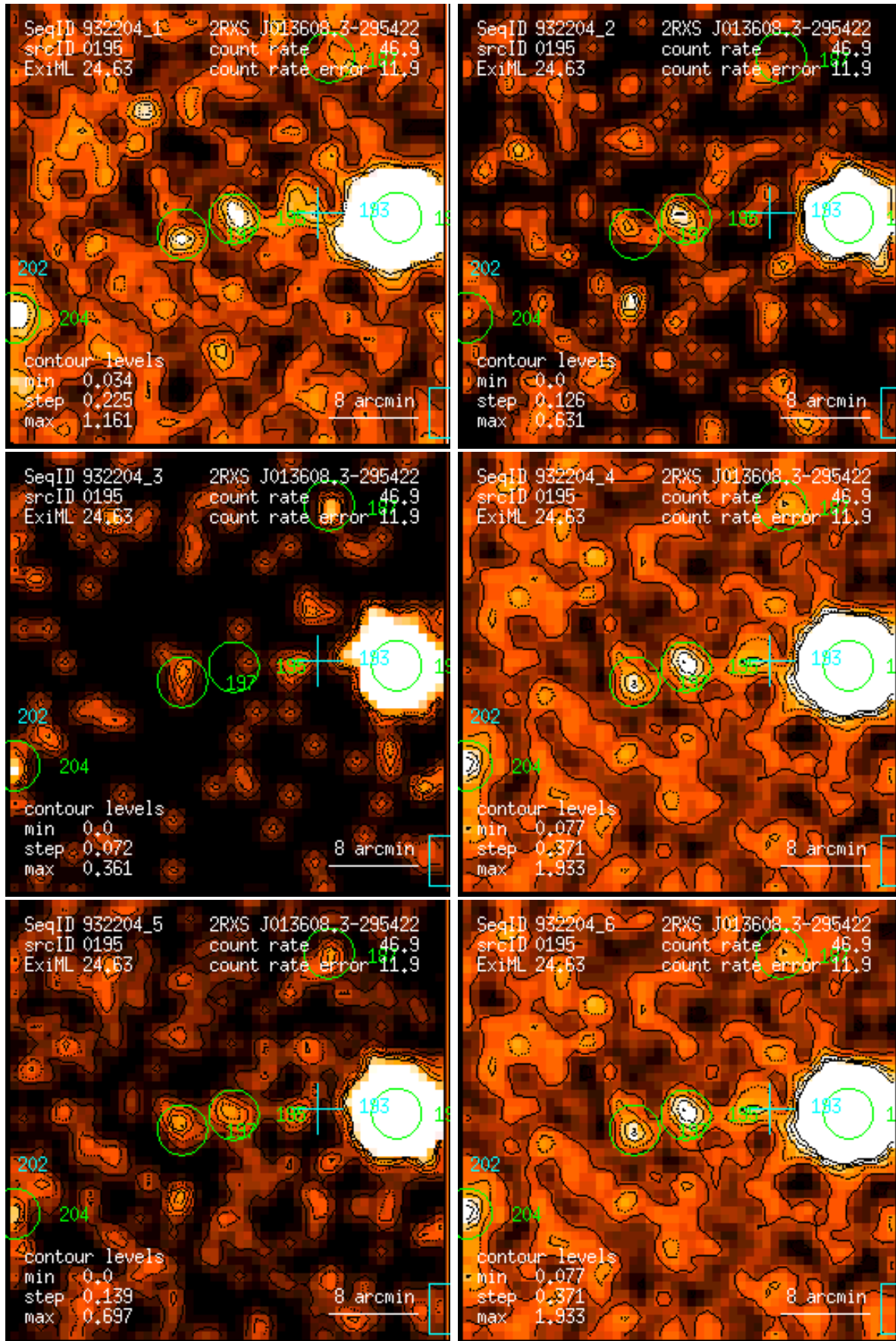
Figure 195: RASS 932204: detection 0195: band rate images, Gaussian filter: (1) PSPC channels 11 – 41, (2) 52 – 90, (3) 91 – 201, (4) 11 – 235, (5) 52 – 201, (6) 11 – 201. Broad band rates in counts/ks. Band rate contour levels in counts/ks/arcmin 2 .
