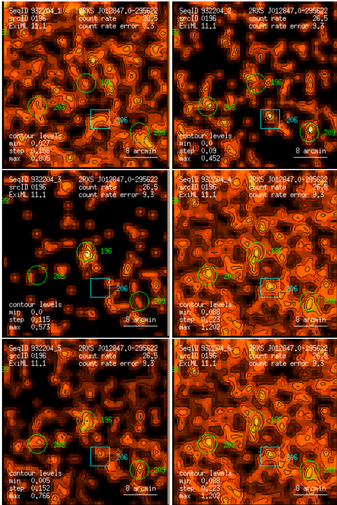
Figure 196: RASS 932204: detection 0196: band rate images, Gaussian filter: (1) PSPC channels 11 – 41, (2) 52 – 90, (3) 91 – 201, (4) 11 – 235, (5) 52 – 201, (6) 11 – 201. Broad band rates in counts/ks. Band rate contour levels in counts/ks/arcmin 2 .
