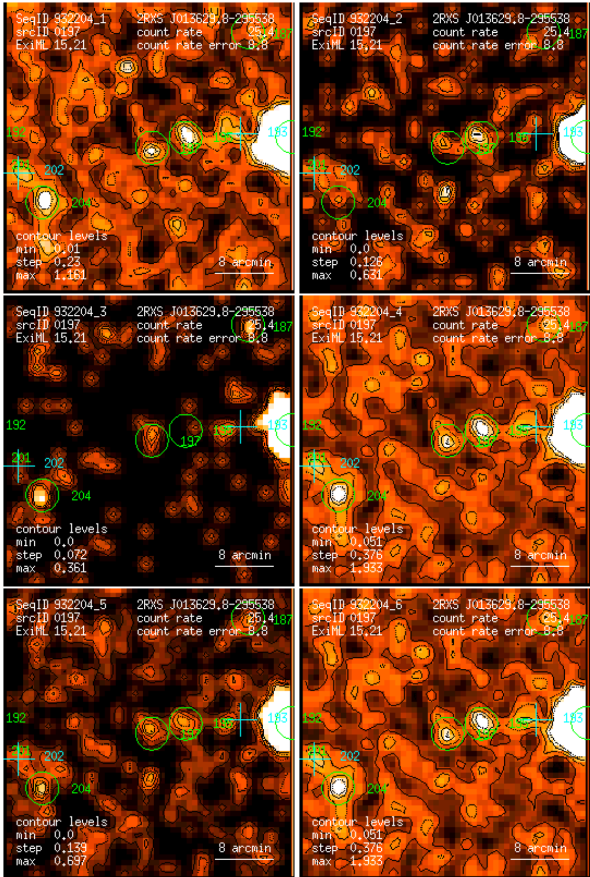
Figure 197: RASS 932204: detection 0197: band rate images, Gaussian filter: (1) PSPC channels 11 – 41, (2) 52 – 90, (3) 91 – 201, (4) 11 – 235, (5) 52 – 201, (6) 11 – 201. Broad band rates in counts/ks. Band rate contour levels in counts/ks/arcmin 2 .
