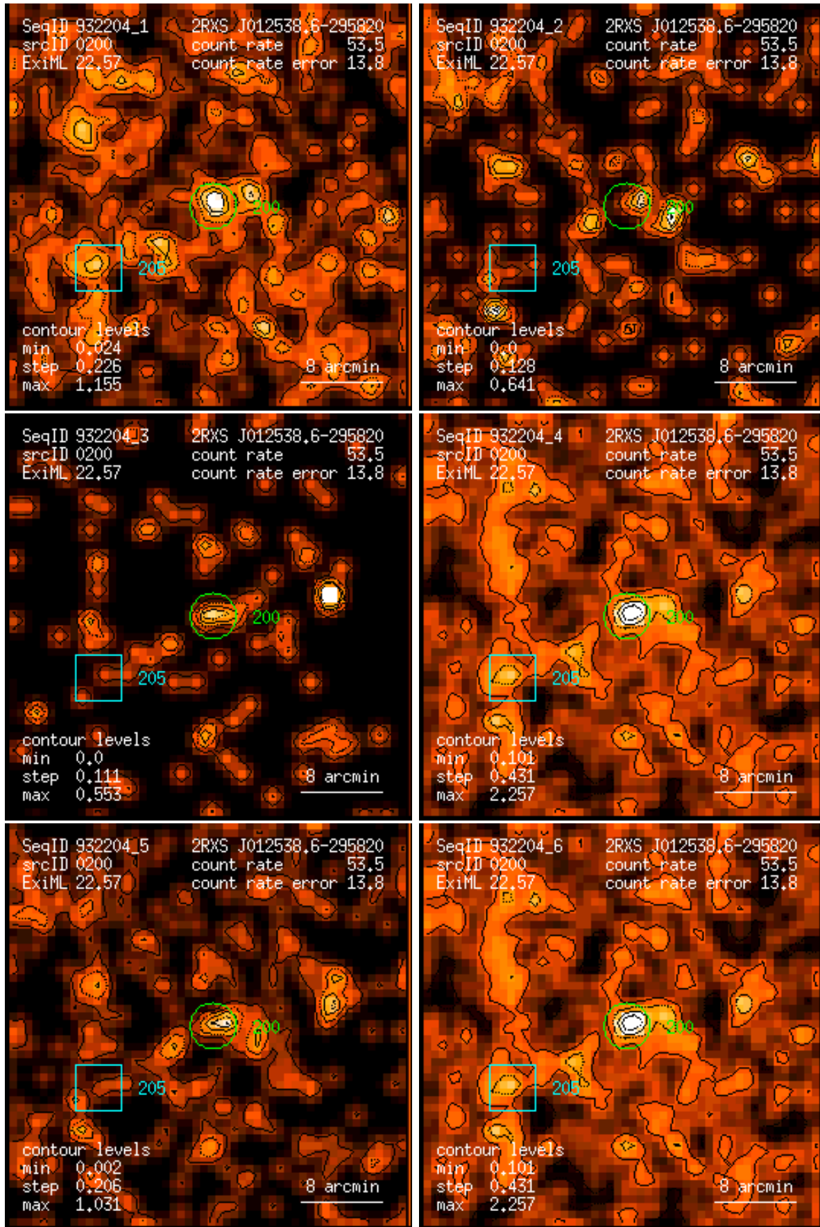
Figure 200: RASS 932204: detection 0200: band rate images, Gaussian filter: (1) PSPC channels 11 – 41, (2) 52 – 90, (3) 91 – 201, (4) 11 – 235, (5) 52 – 201, (6) 11 – 201. Broad band rates in counts/ks. Band rate contour levels in counts/ks/arcmin 2 .
