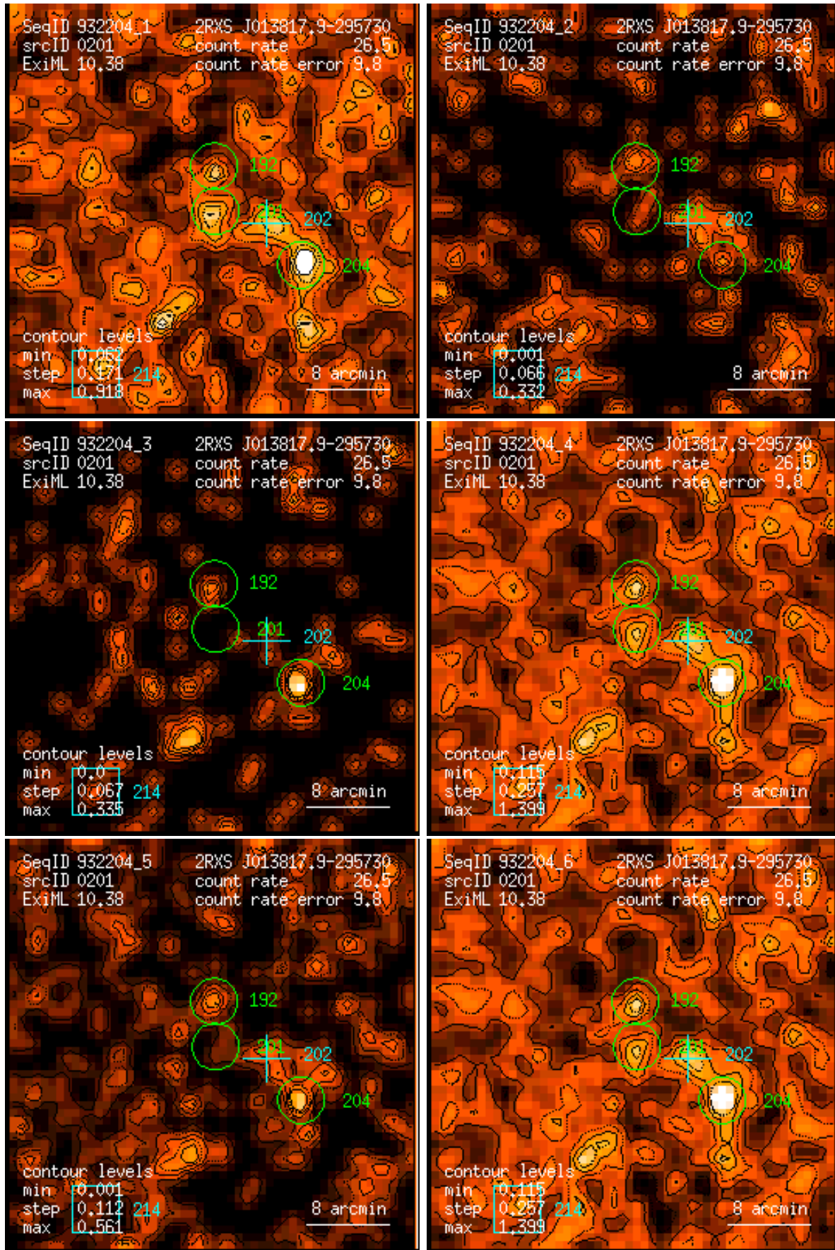
Figure 201: RASS 932204: detection 0201: band rate images, Gaussian filter: (1) PSPC channels 11 – 41, (2) 52 – 90, (3) 91 – 201, (4) 11 – 235, (5) 52 – 201, (6) 11 – 201. Broad band rates in counts/ks. Band rate contour levels in counts/ks/arcmin 2 .
