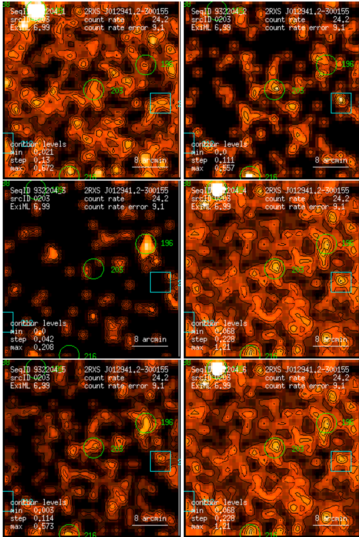
Figure 203: RASS 932204: detection 0203: band rate images, Gaussian filter: (1) PSPC channels 11 – 41, (2) 52 – 90, (3) 91 – 201, (4) 11 – 235, (5) 52 – 201, (6) 11 – 201. Broad band rates in counts/ks. Band rate contour levels in counts/ks/arcmin 2 .
