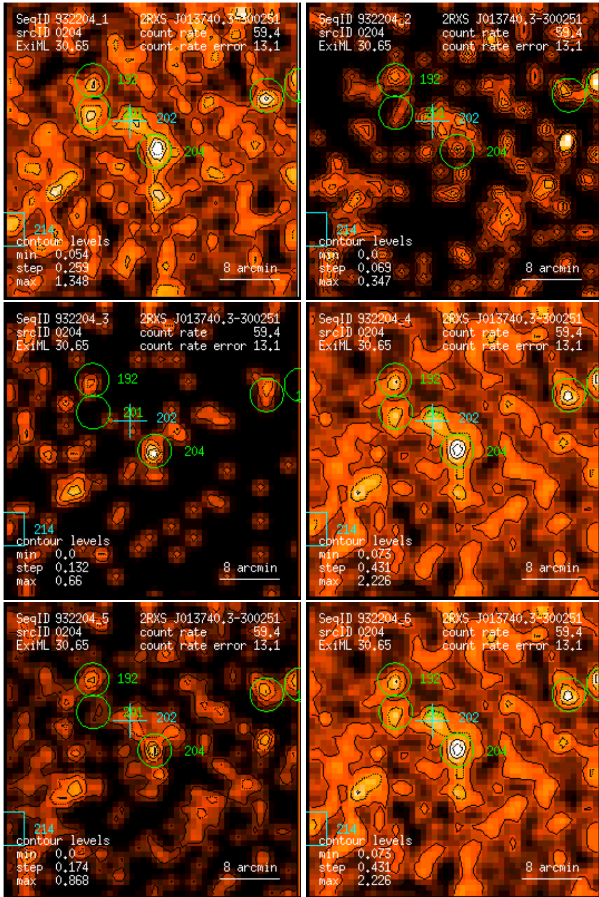
Figure 204: RASS 932204: detection 0204: band rate images, Gaussian filter: (1) PSPC channels 11 – 41, (2) 52 – 90, (3) 91 – 201, (4) 11 – 235, (5) 52 – 201, (6) 11 – 201. Broad band rates in counts/ks. Band rate contour levels in counts/ks/arcmin 2 .
