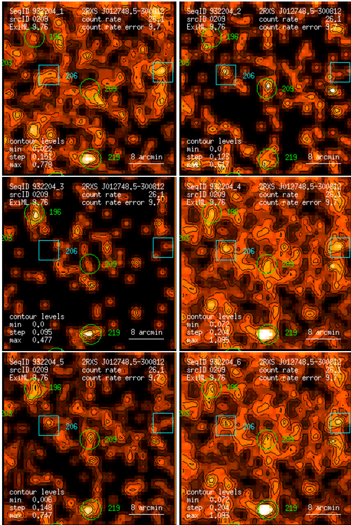
Figure 209: RASS 932204: detection 0209: band rate images, Gaussian filter: (1) PSPC channels 11 – 41, (2) 52 – 90, (3) 91 – 201, (4) 11 – 235, (5) 52 – 201, (6) 11 – 201. Broad band rates in counts/ks. Band rate contour levels in counts/ks/arcmin 2 .
