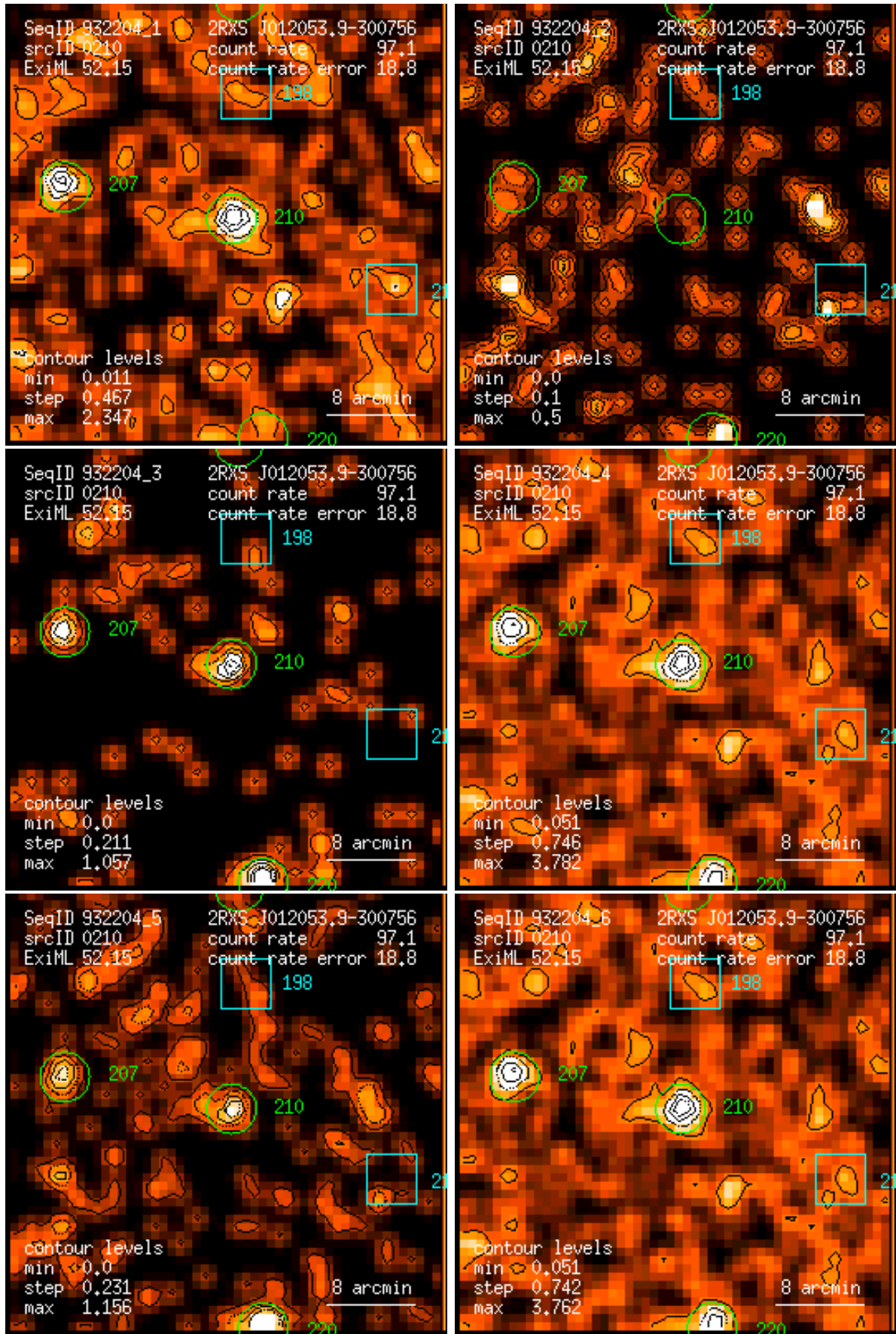
Figure 210: RASS 932204: detection 0210: band rate images, Gaussian filter: (1) PSPC channels 11 – 41, (2) 52 – 90, (3) 91 – 201, (4) 11 – 235, (5) 52 – 201, (6) 11 – 201. Broad band rates in counts/ks. Band rate contour levels in counts/ks/arcmin 2 .
