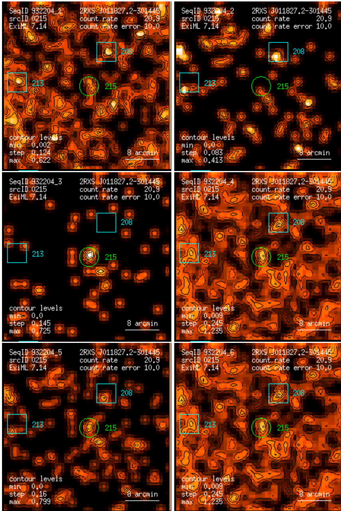
Figure 215: RASS 932204: detection 0215: band rate images, Gaussian filter: (1) PSPC channels 11 – 41, (2) 52 – 90, (3) 91 – 201, (4) 11 – 235, (5) 52 – 201, (6) 11 – 201. Broad band rates in counts/ks. Band rate contour levels in counts/ks/arcmin 2 .
