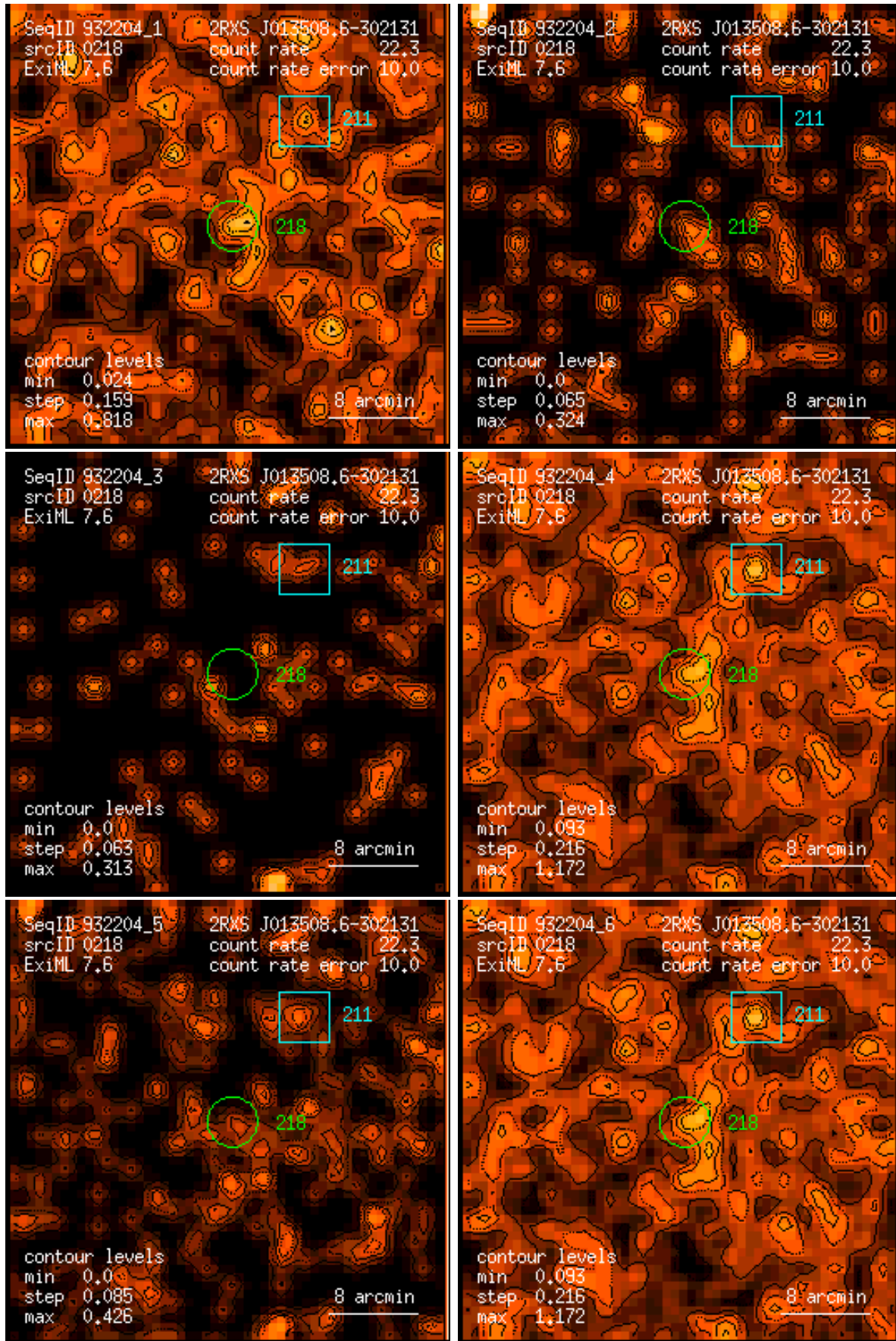
Figure 218: RASS 932204: detection 0218: band rate images, Gaussian filter: (1) PSPC channels 11 – 41, (2) 52 – 90, (3) 91 – 201, (4) 11 – 235, (5) 52 – 201, (6) 11 – 201. Broad band rates in counts/ks. Band rate contour levels in counts/ks/arcmin 2 .
