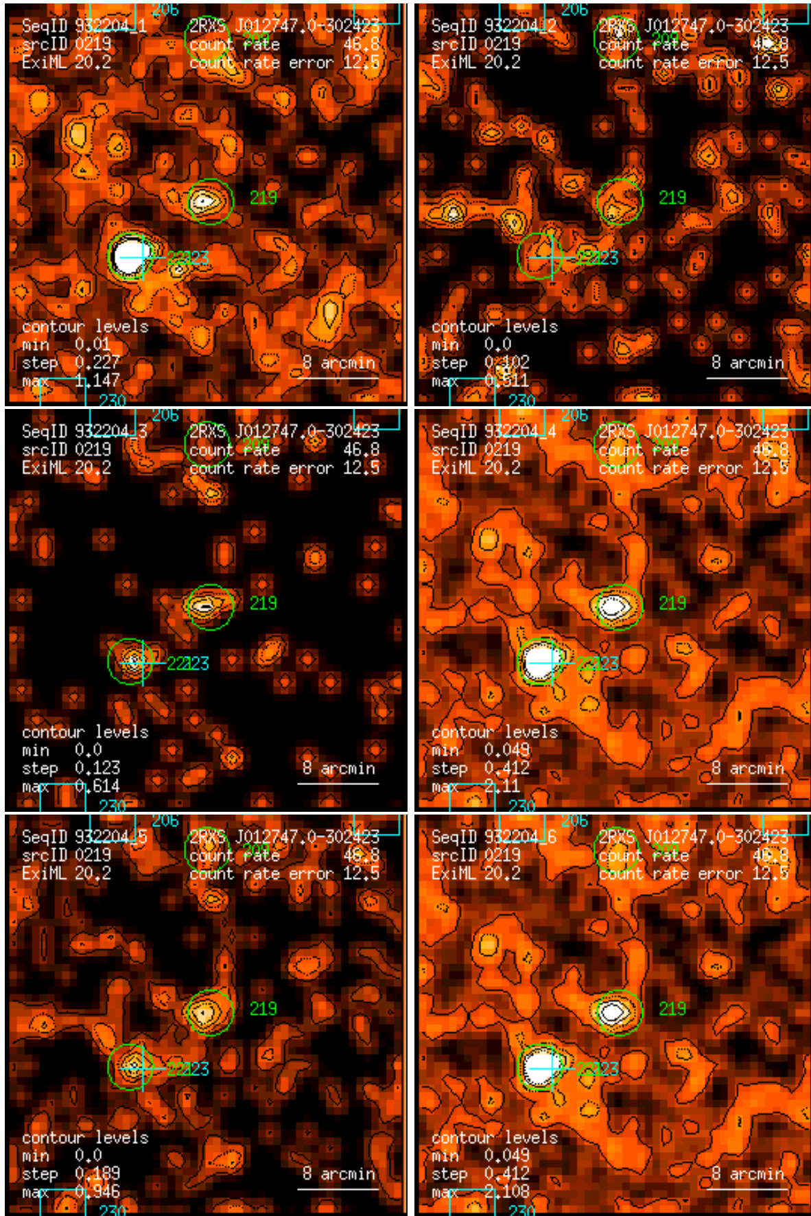
Figure 219: RASS 932204: detection 0219: band rate images, Gaussian filter: (1) PSPC channels 11 – 41, (2) 52 – 90, (3) 91 – 201, (4) 11 – 235, (5) 52 – 201, (6) 11 – 201. Broad band rates in counts/ks. Band rate contour levels in counts/ks/arcmin 2 .
