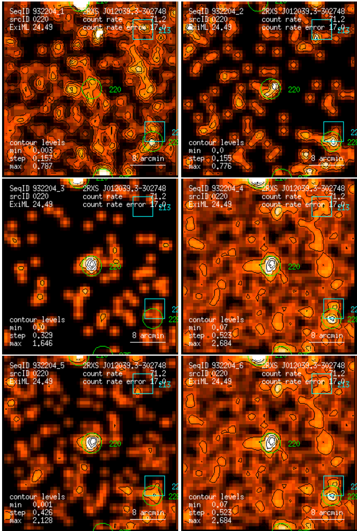
Figure 220: RASS 932204: detection 0220: band rate images, Gaussian filter: (1) PSPC channels 11 – 41, (2) 52 – 90, (3) 91 – 201, (4) 11 – 235, (5) 52 – 201, (6) 11 – 201. Broad band rates in counts/ks. Band rate contour levels in counts/ks/arcmin 2 .
