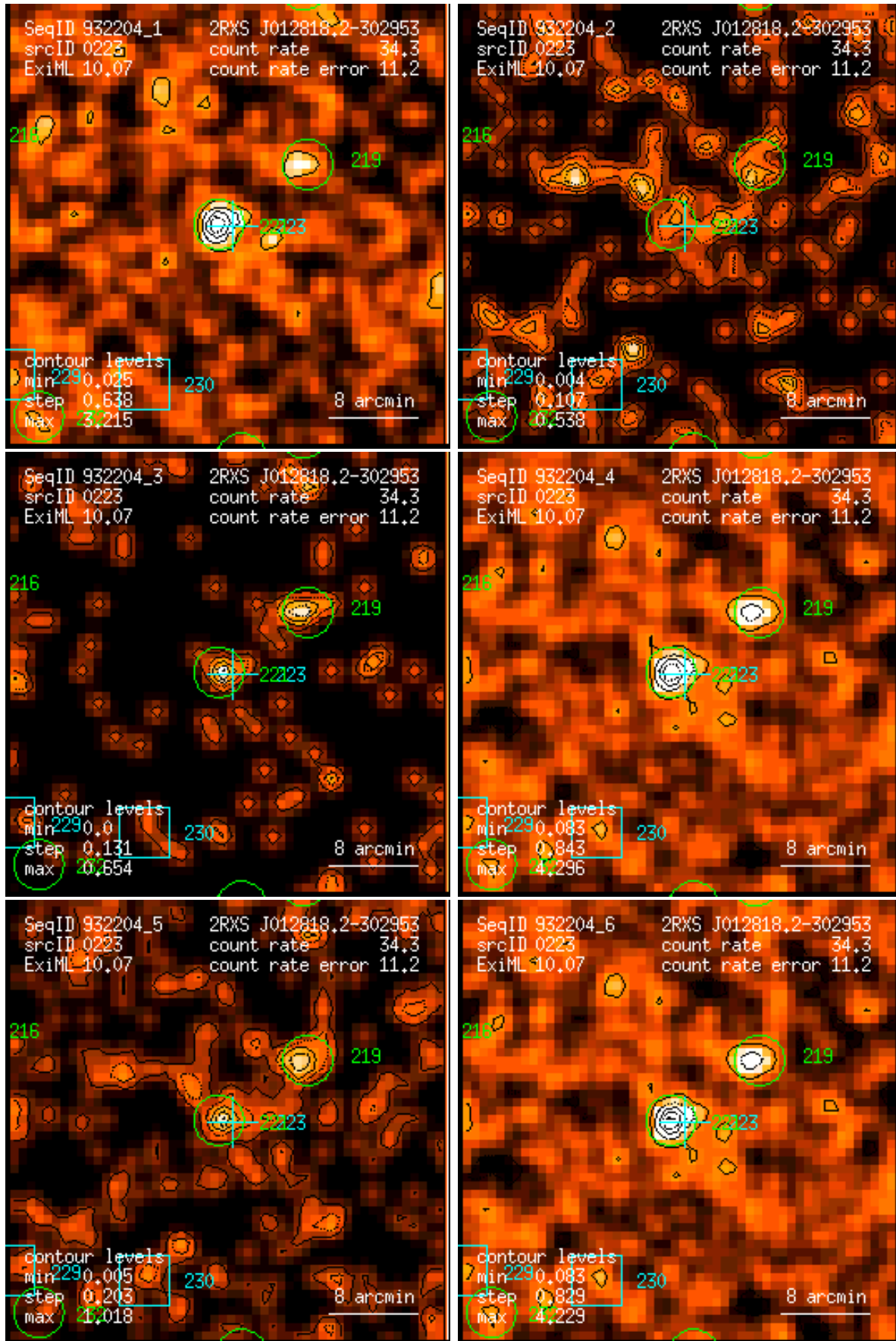
Figure 223: RASS 932204: detection 0223: band rate images, Gaussian filter: (1) PSPC channels 11 – 41, (2) 52 – 90, (3) 91 – 201, (4) 11 – 235, (5) 52 – 201, (6) 11 – 201. Broad band rates in counts/ks. Band rate contour levels in counts/ks/arcmin 2 .
