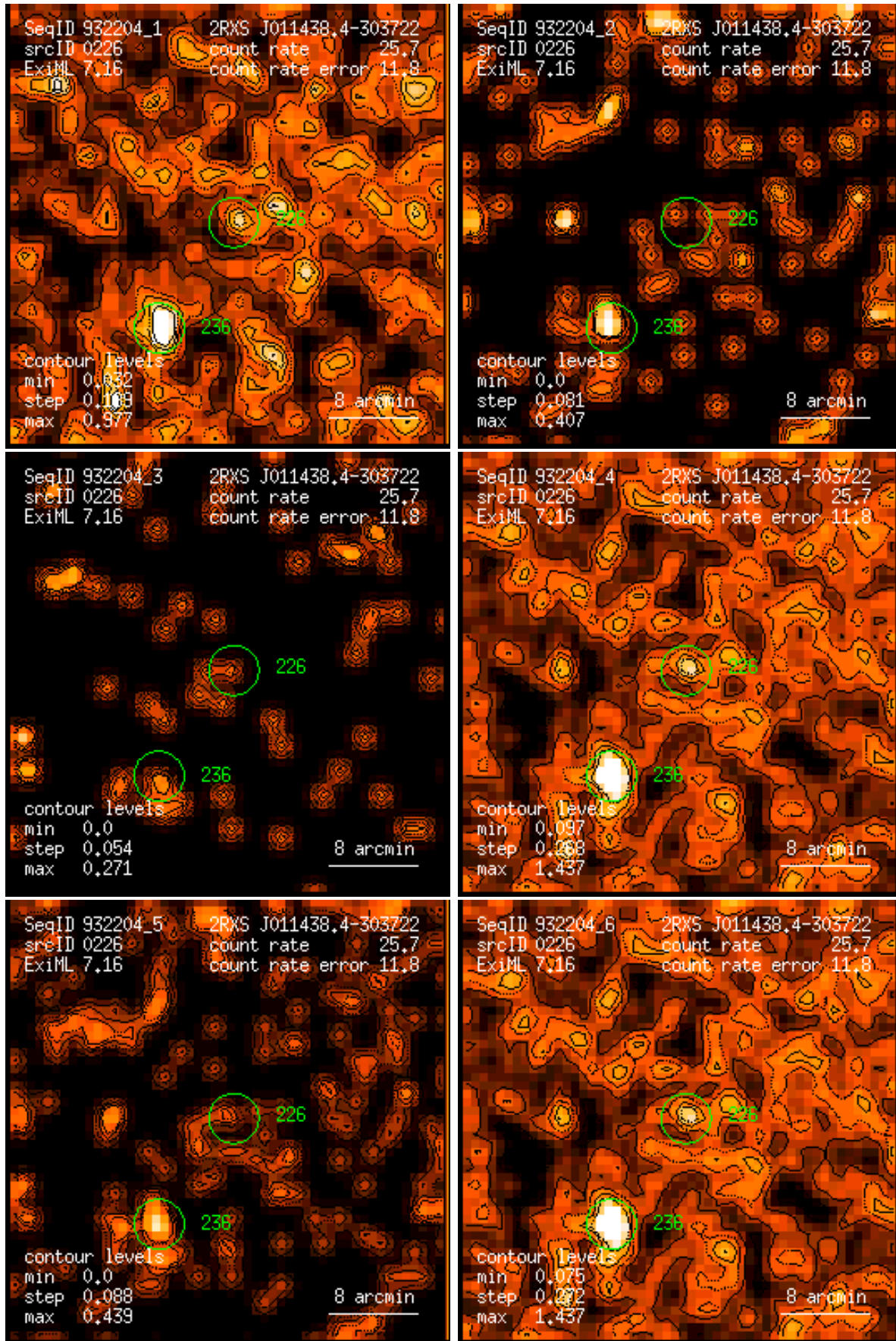
Figure 226: RASS 932204: detection 0226: band rate images, Gaussian filter: (1) PSPC channels 11 – 41, (2) 52 – 90, (3) 91 – 201, (4) 11 – 235, (5) 52 – 201, (6) 11 – 201. Broad band rates in counts/ks. Band rate contour levels in counts/ks/arcmin 2 .
