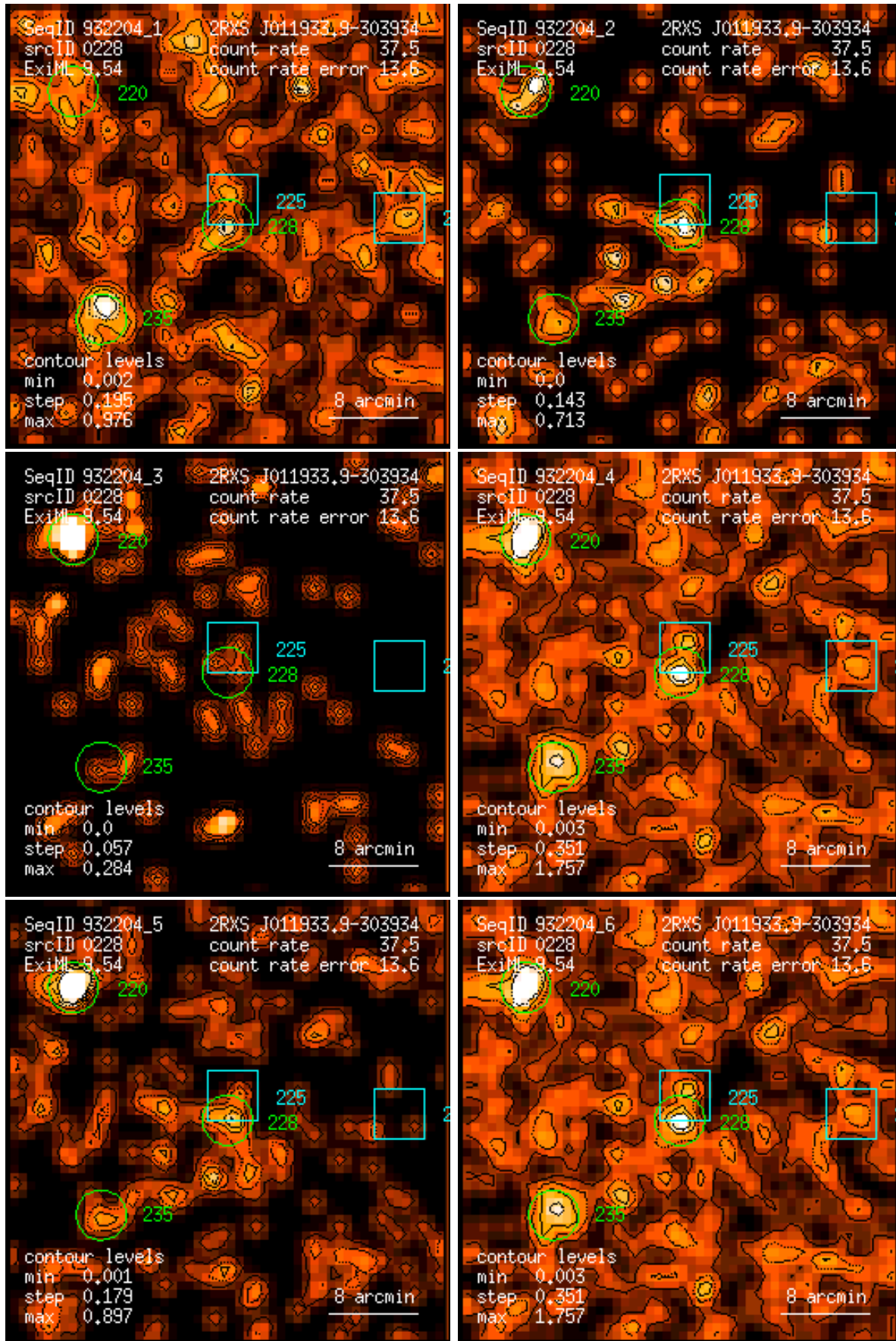
Figure 228: RASS 932204: detection 0228: band rate images, Gaussian filter: (1) PSPC channels 11 – 41, (2) 52 – 90, (3) 91 – 201, (4) 11 – 235, (5) 52 – 201, (6) 11 – 201. Broad band rates in counts/ks. Band rate contour levels in counts/ks/arcmin 2 .
