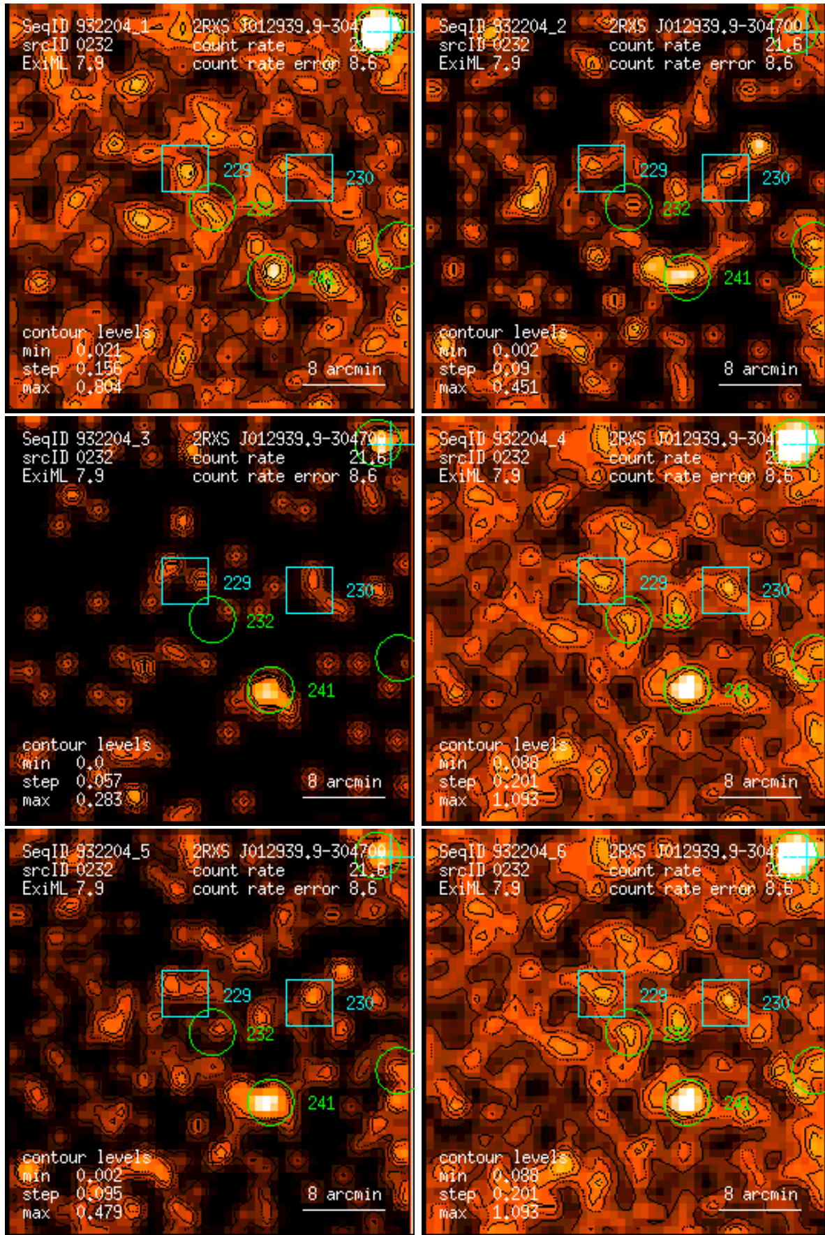
Figure 232: RASS 932204: detection 0232: band rate images, Gaussian filter: (1) PSPC channels 11 – 41, (2) 52 – 90, (3) 91 – 201, (4) 11 – 235, (5) 52 – 201, (6) 11 – 201. Broad band rates in counts/ks. Band rate contour levels in counts/ks/arcmin 2 .
