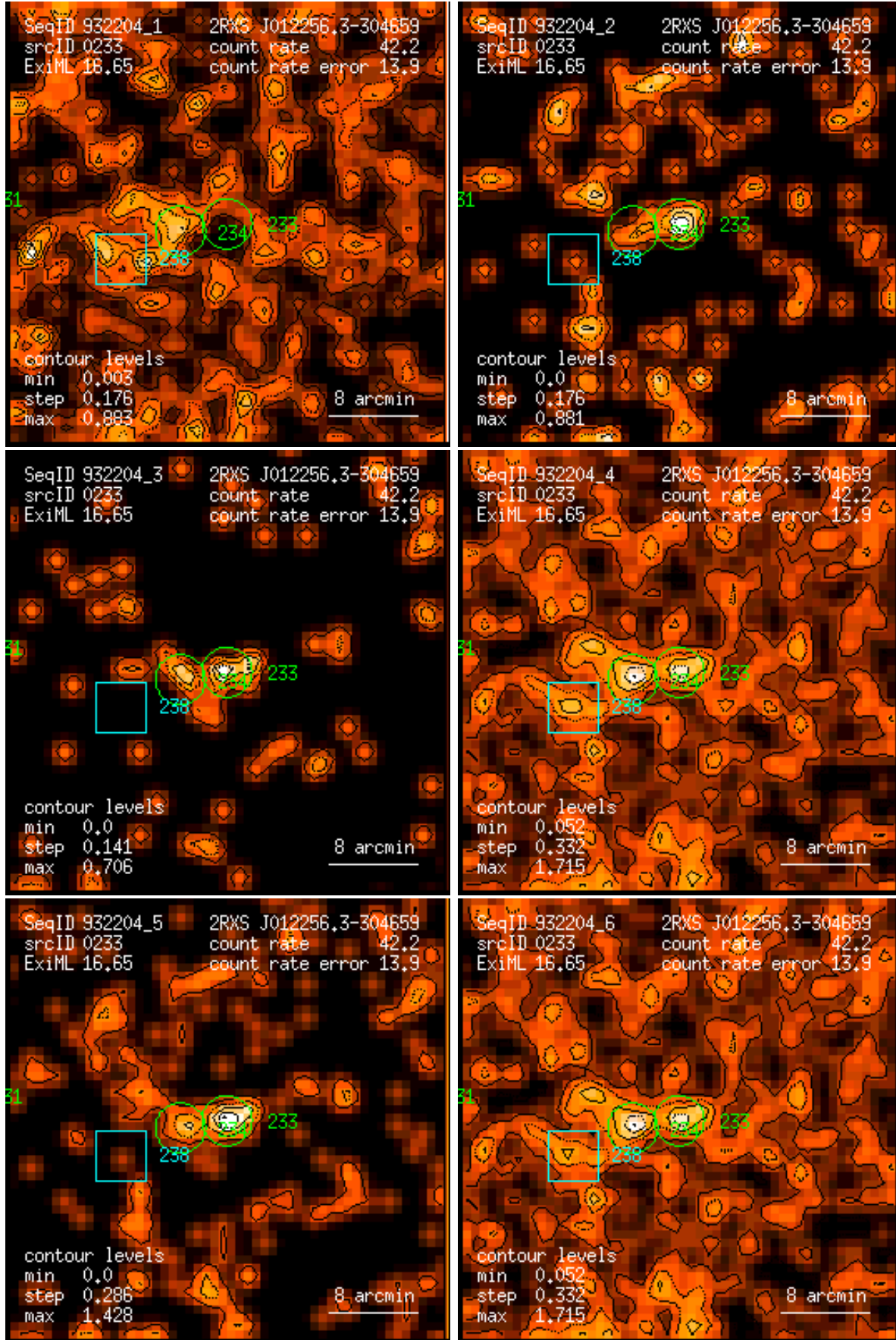
Figure 233: RASS 932204: detection 0233: band rate images, Gaussian filter: (1) PSPC channels 11 – 41, (2) 52 – 90, (3) 91 – 201, (4) 11 – 235, (5) 52 – 201, (6) 11 – 201. Broad band rates in counts/ks. Band rate contour levels in counts/ks/arcmin 2 .
