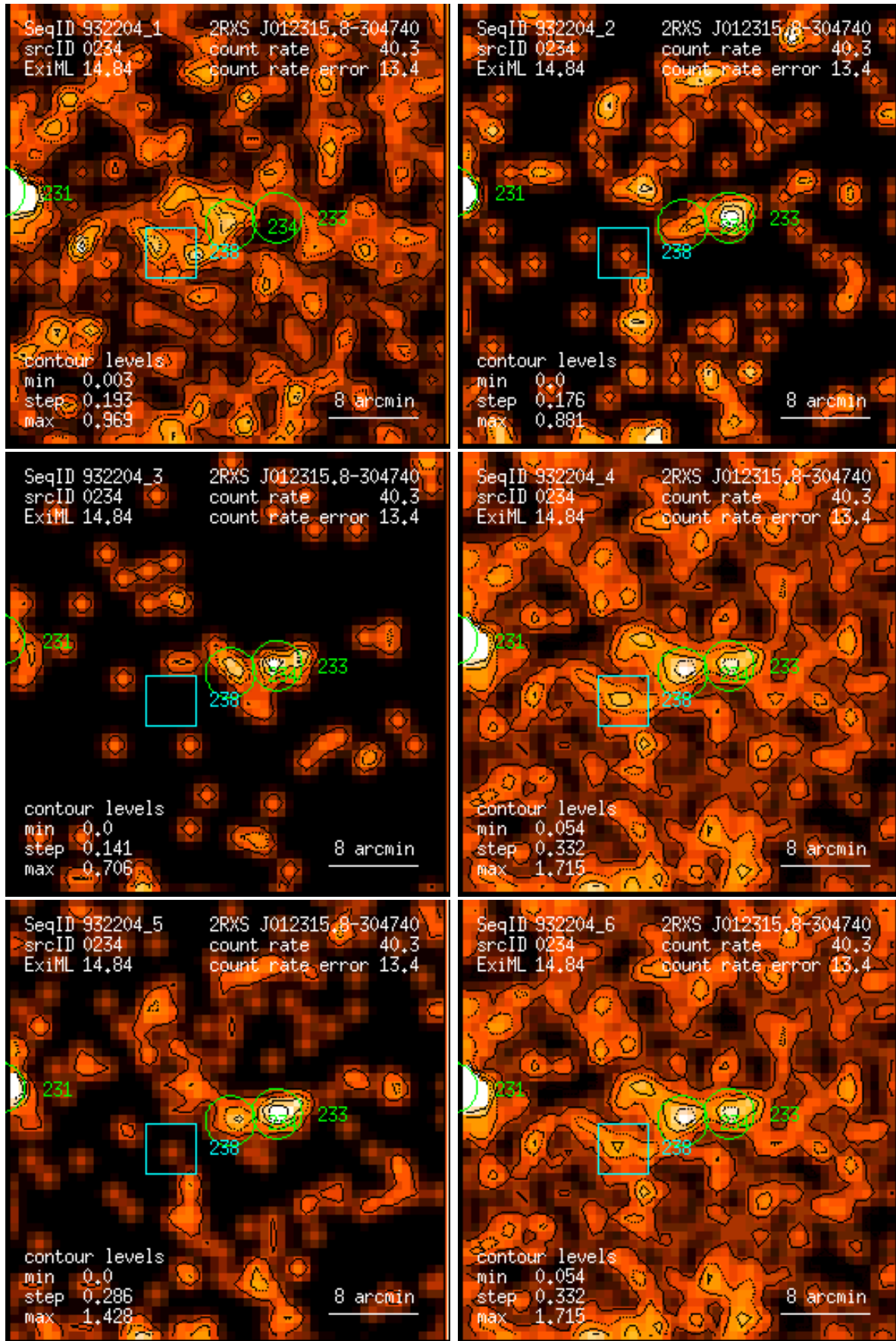
Figure 234: RASS 932204: detection 0234: band rate images, Gaussian filter: (1) PSPC channels 11 – 41, (2) 52 – 90, (3) 91 – 201, (4) 11 – 235, (5) 52 – 201, (6) 11 – 201. Broad band rates in counts/ks. Band rate contour levels in counts/ks/arcmin 2 .
