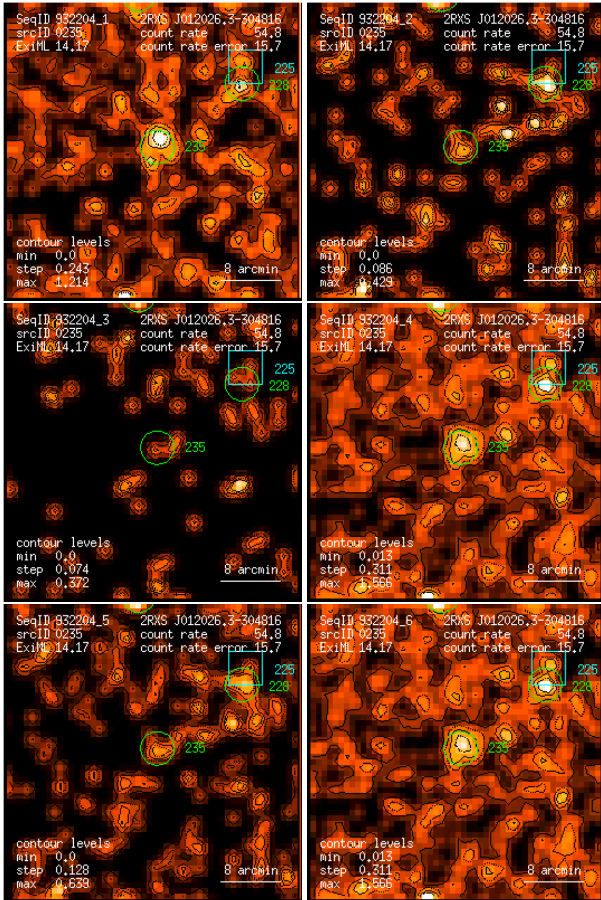
Figure 235: RASS 932204: detection 0235: band rate images, Gaussian filter: (1) PSPC channels 11 – 41, (2) 52 – 90, (3) 91 – 201, (4) 11 – 235, (5) 52 – 201, (6) 11 – 201. Broad band rates in counts/ks. Band rate contour levels in counts/ks/arcmin 2 .
