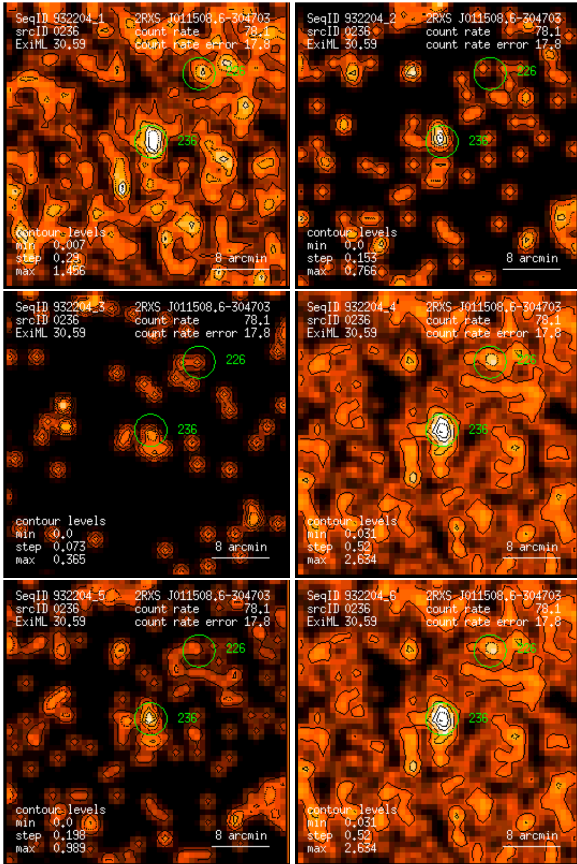
Figure 236: RASS 932204: detection 0236: band rate images, Gaussian filter: (1) PSPC channels 11 – 41, (2) 52 – 90, (3) 91 – 201, (4) 11 – 235, (5) 52 – 201, (6) 11 – 201. Broad band rates in counts/ks. Band rate contour levels in counts/ks/arcmin 2 .
