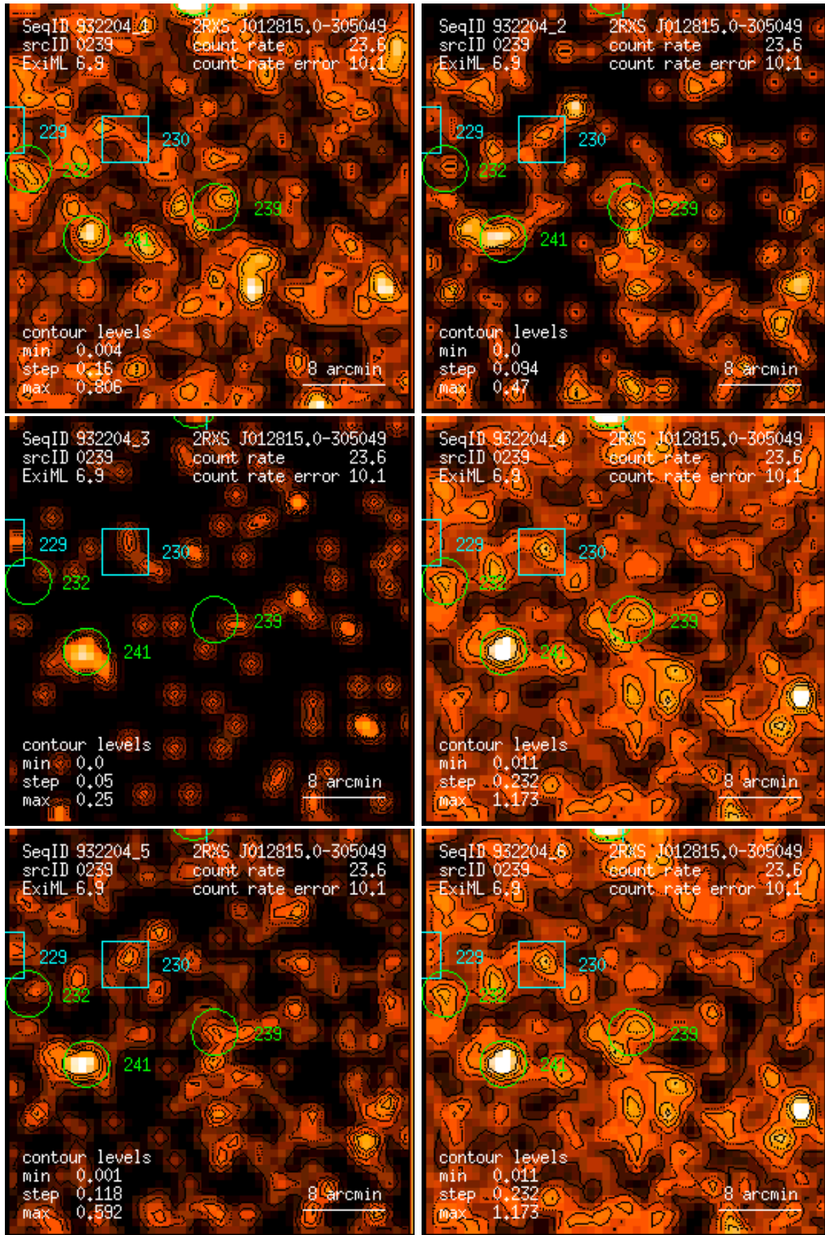
Figure 239: RASS 932204: detection 0239: band rate images, Gaussian filter: (1) PSPC channels 11 – 41, (2) 52 – 90, (3) 91 – 201, (4) 11 – 235, (5) 52 – 201, (6) 11 – 201. Broad band rates in counts/ks. Band rate contour levels in counts/ks/arcmin 2 .
