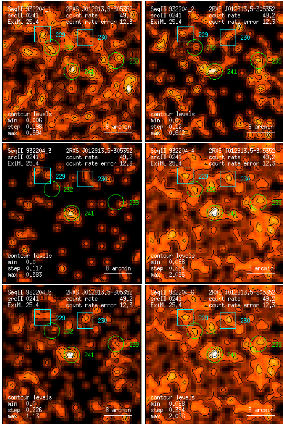
Figure 241: RASS 932204: detection 0241: band rate images, Gaussian filter: (1) PSPC channels 11 – 41, (2) 52 – 90, (3) 91 – 201, (4) 11 – 235, (5) 52 – 201, (6) 11 – 201. Broad band rates in counts/ks. Band rate contour levels in counts/ks/arcmin 2 .
