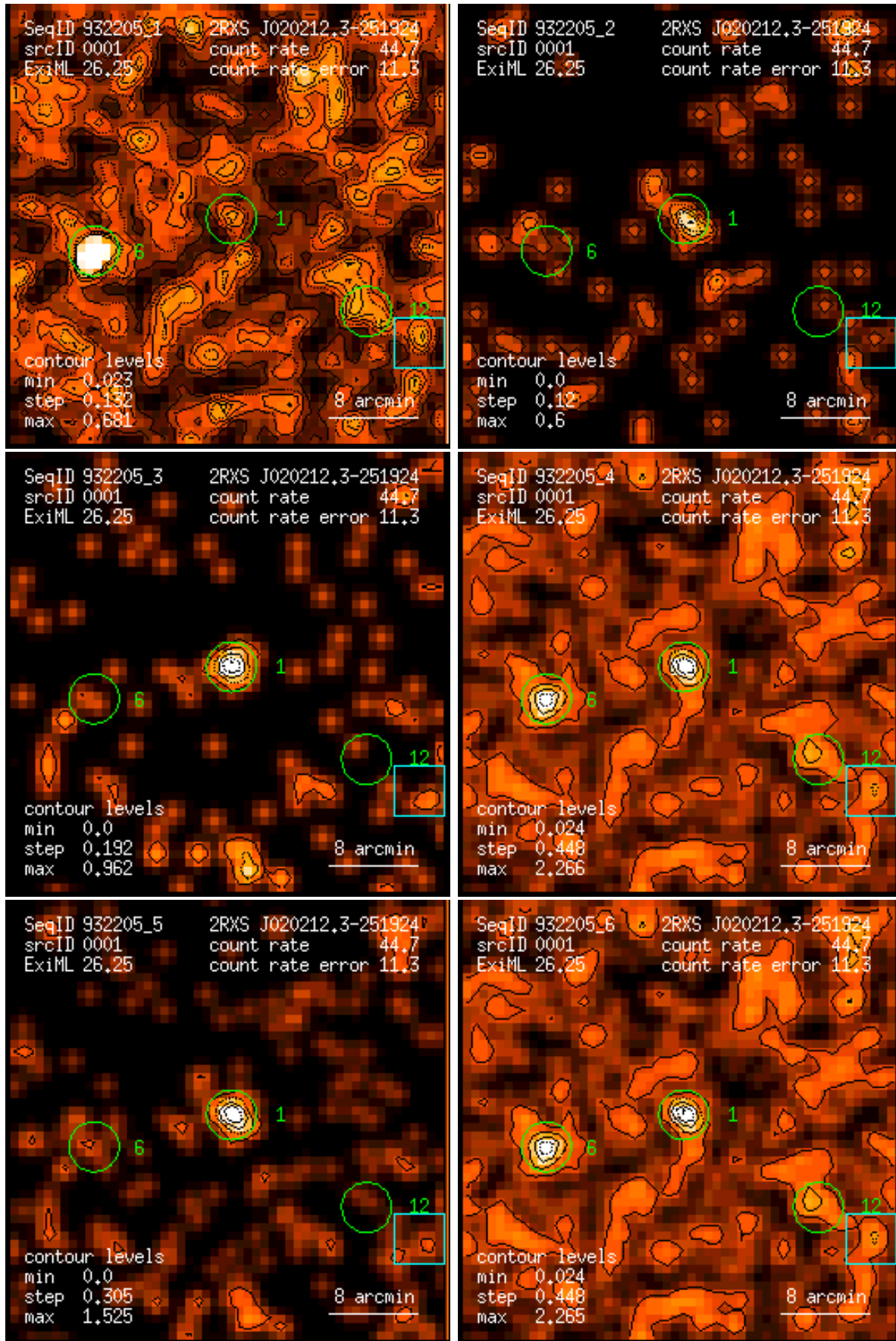
Figure 1: RASS 932205: detection 0001: band rate images, Gaussian filter: (1) PSPC channels 11 – 41, (2) 52 – 90, (3) 91 – 201, (4) 11 – 235, (5) 52 – 201, (6) 11 – 201. Broad band rates in counts/ks. Band rate contour levels in counts/ks/arcmin 2 .
