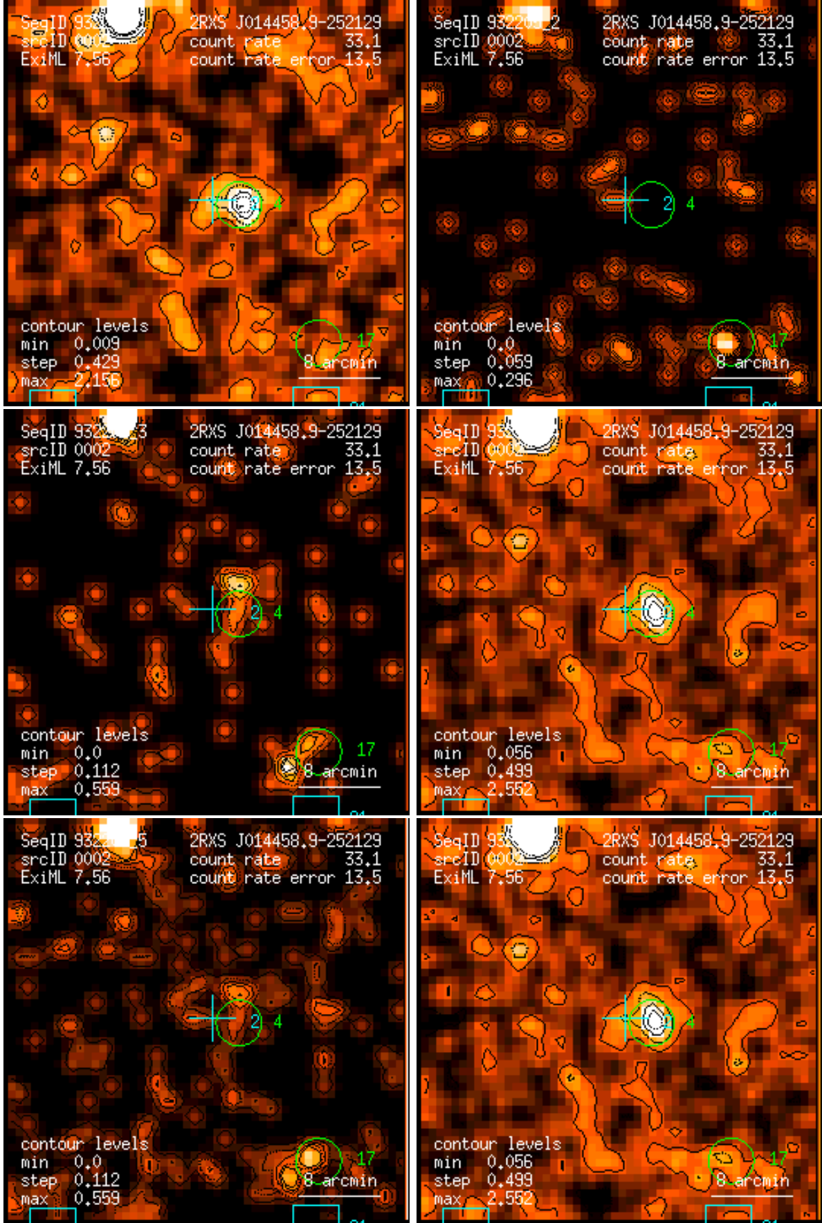
Figure 2: RASS 932205: detection 0002: band rate images, Gaussian filter: (1) PSPC channels 11 – 41, (2) 52 – 90, (3) 91 – 201, (4) 11 – 235, (5) 52 – 201, (6) 11 – 201. Broad band rates in counts/ks. Band rate contour levels in counts/ks/arcmin 2 .
