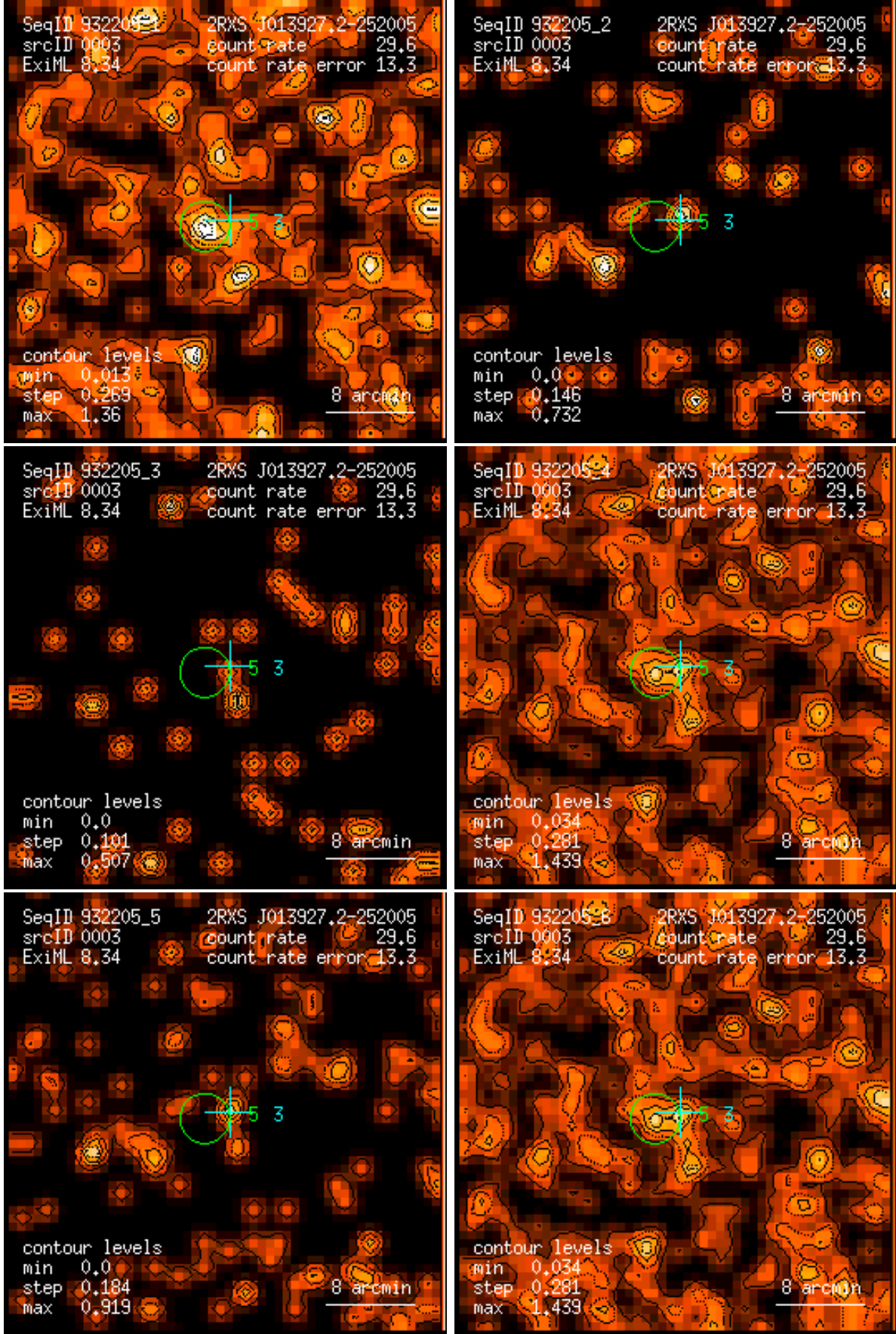
Figure 3: RASS 932205: detection 0003: band rate images, Gaussian filter: (1) PSPC channels 11 – 41, (2) 52 – 90, (3) 91 – 201, (4) 11 – 235, (5) 52 – 201, (6) 11 – 201. Broad band rates in counts/ks. Band rate contour levels in counts/ks/arcmin 2 .
