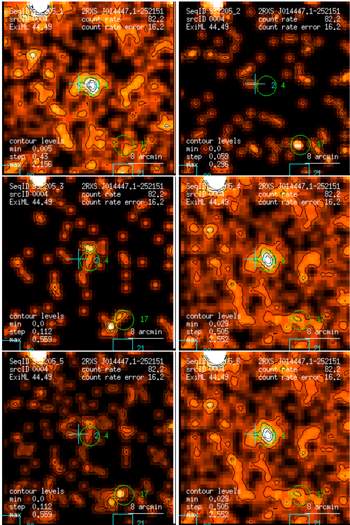
Figure 4: RASS 932205: detection 0004: band rate images, Gaussian filter: (1) PSPC channels 11 – 41, (2) 52 – 90, (3) 91 – 201, (4) 11 – 235, (5) 52 – 201, (6) 11 – 201. Broad band rates in counts/ks. Band rate contour levels in counts/ks/arcmin 2 .
