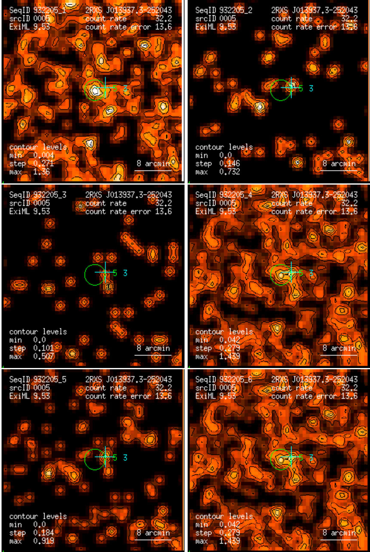
Figure 5: RASS 932205: detection 0005: band rate images, Gaussian filter: (1) PSPC channels 11 – 41, (2) 52 – 90, (3) 91 – 201, (4) 11 – 235, (5) 52 – 201, (6) 11 – 201. Broad band rates in counts/ks. Band rate contour levels in counts/ks/arcmin 2 .
