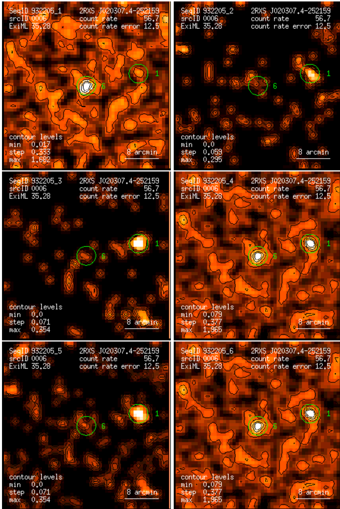
Figure 6: RASS 932205: detection 0006: band rate images, Gaussian filter: (1) PSPC channels 11 – 41, (2) 52 – 90, (3) 91 – 201, (4) 11 – 235, (5) 52 – 201, (6) 11 – 201. Broad band rates in counts/ks. Band rate contour levels in counts/ks/arcmin 2 .
