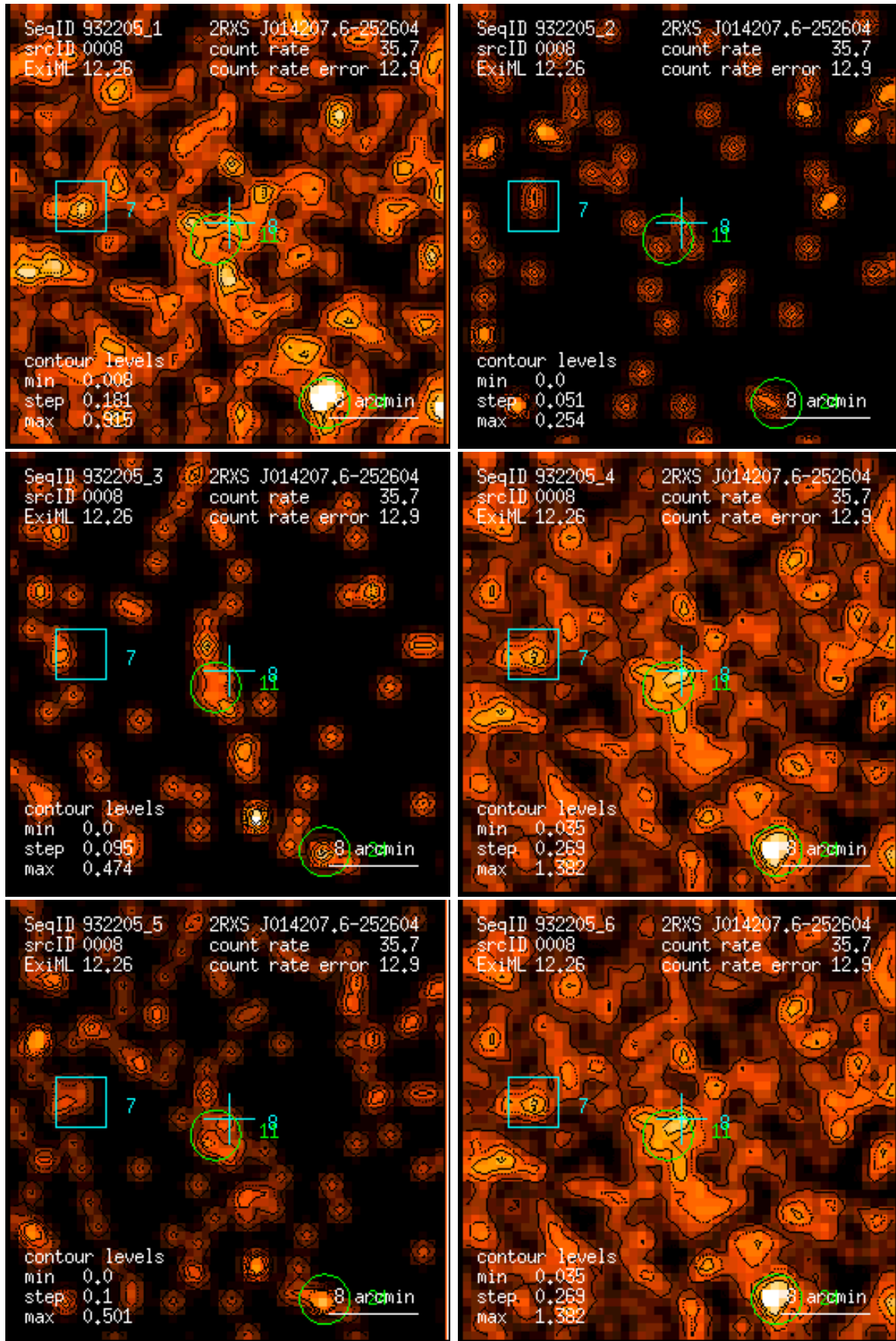
Figure 8: RASS 932205: detection 0008: band rate images, Gaussian filter: (1) PSPC channels 11 – 41, (2) 52 – 90, (3) 91 – 201, (4) 11 – 235, (5) 52 – 201, (6) 11 – 201. Broad band rates in counts/ks. Band rate contour levels in counts/ks/arcmin 2 .
