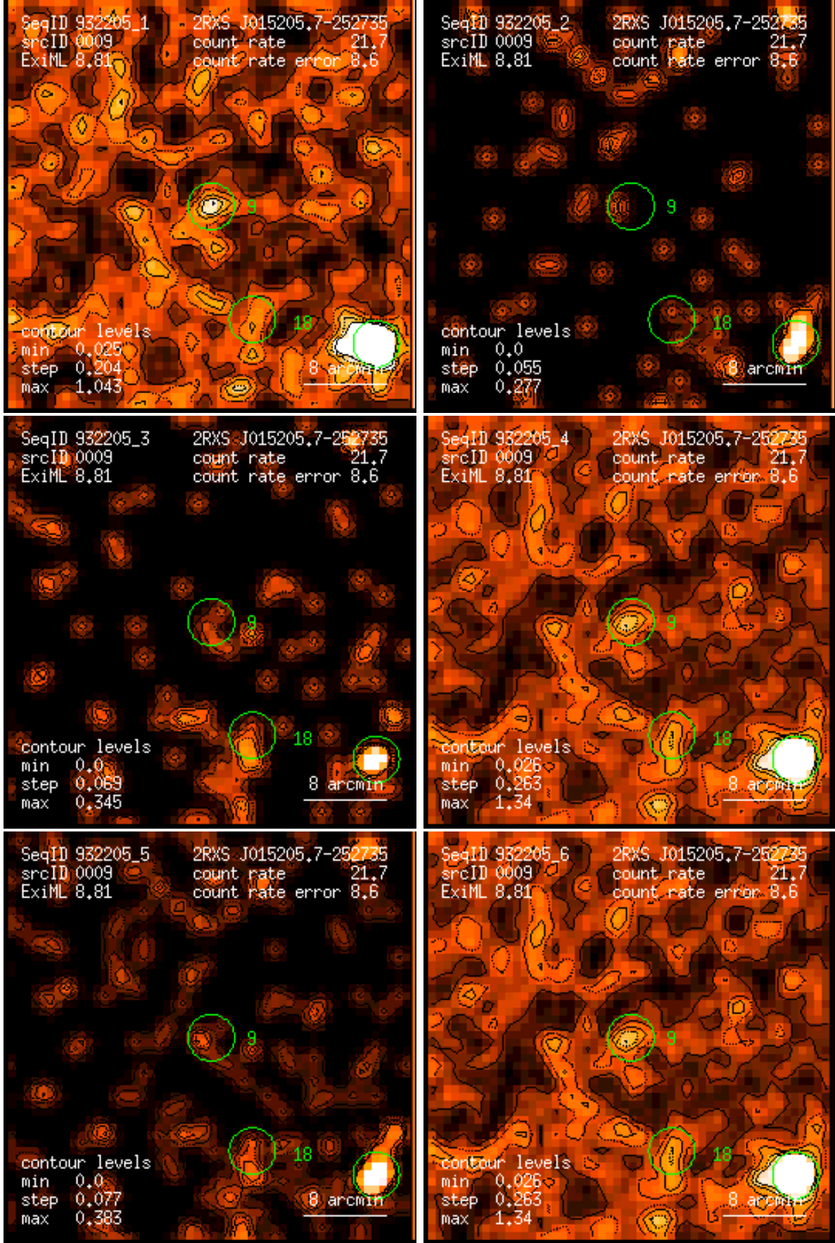
Figure 9: RASS 932205: detection 0009: band rate images, Gaussian filter: (1) PSPC channels 11 – 41, (2) 52 – 90, (3) 91 – 201, (4) 11 – 235, (5) 52 – 201, (6) 11 – 201. Broad band rates in counts/ks. Band rate contour levels in counts/ks/arcmin 2 .
