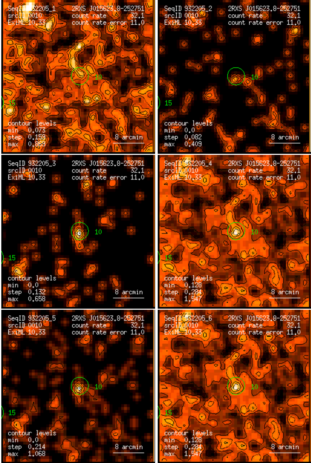
Figure 10: RASS 932205: detection 0010: band rate images, Gaussian filter: (1) PSPC channels 11 – 41, (2) 52 – 90, (3) 91 – 201, (4) 11 – 235, (5) 52 – 201, (6) 11 – 201. Broad band rates in counts/ks. Band rate contour levels in counts/ks/arcmin 2 .
