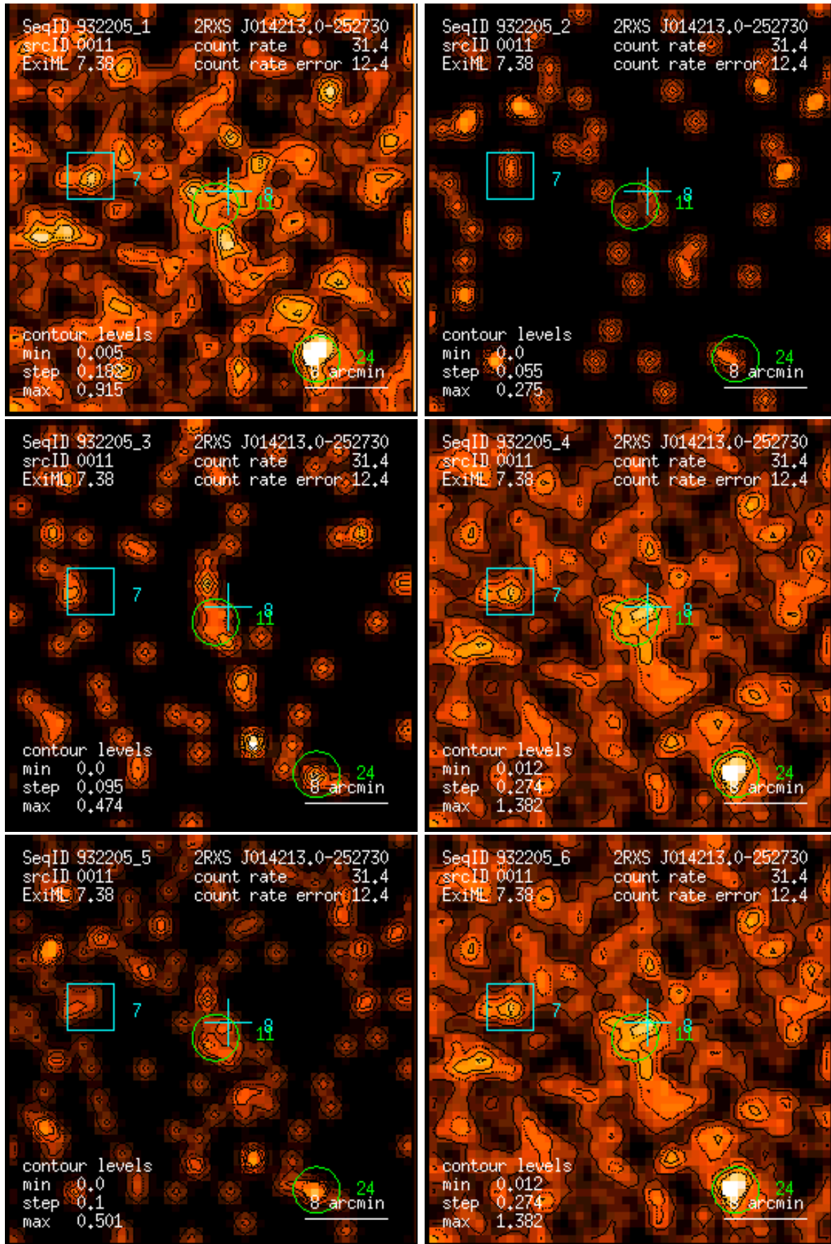
Figure 11: RASS 932205: detection 0011: band rate images, Gaussian filter: (1) PSPC channels 11 – 41, (2) 52 – 90, (3) 91 – 201, (4) 11 – 235, (5) 52 – 201, (6) 11 – 201. Broad band rates in counts/ks. Band rate contour levels in counts/ks/arcmin 2 .
