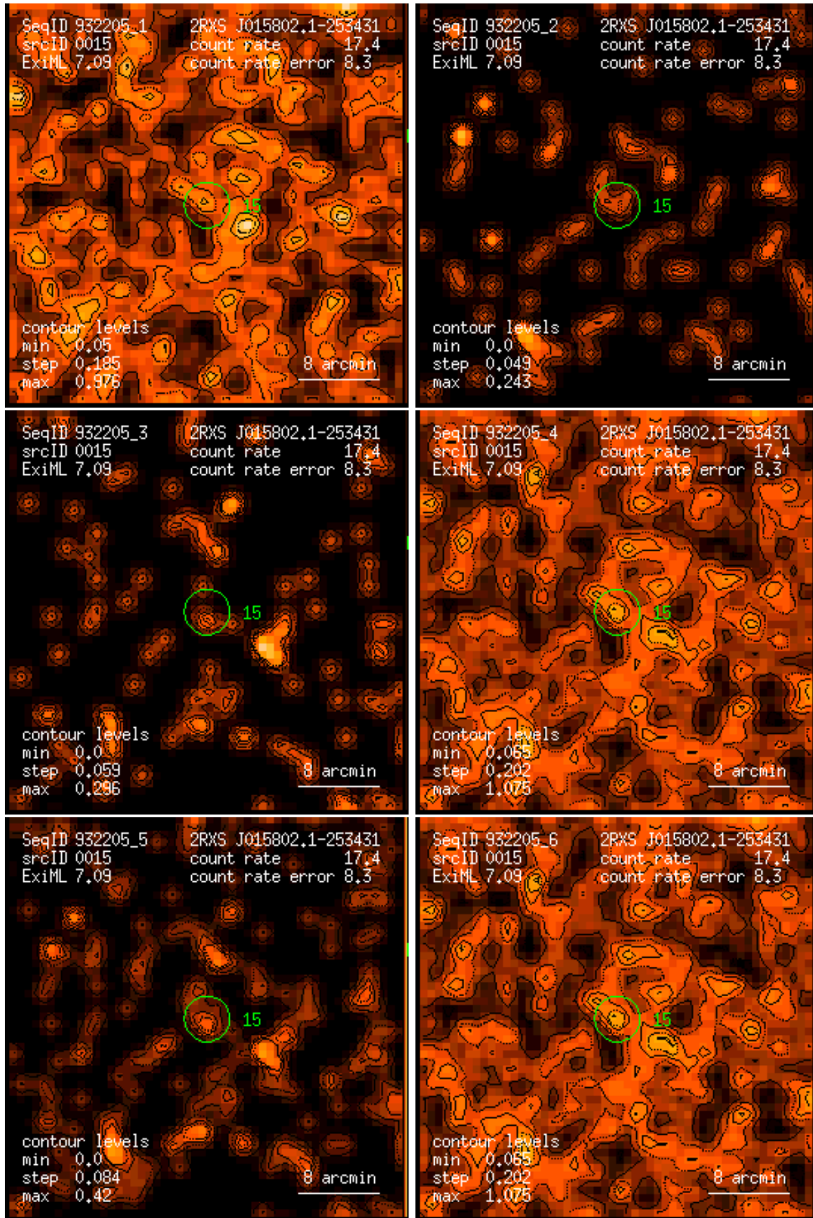
Figure 15: RASS 932205: detection 0015: band rate images, Gaussian filter: (1) PSPC channels 11 – 41, (2) 52 – 90, (3) 91 – 201, (4) 11 – 235, (5) 52 – 201, (6) 11 – 201. Broad band rates in counts/ks. Band rate contour levels in counts/ks/arcmin 2 .
