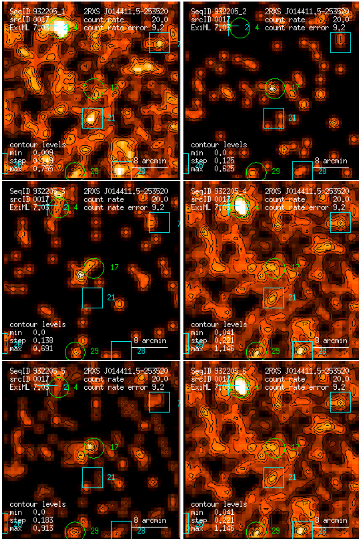
Figure 17: RASS 932205: detection 0017: band rate images, Gaussian filter: (1) PSPC channels 11 – 41, (2) 52 – 90, (3) 91 – 201, (4) 11 – 235, (5) 52 – 201, (6) 11 – 201. Broad band rates in counts/ks. Band rate contour levels in counts/ks/arcmin 2 .
